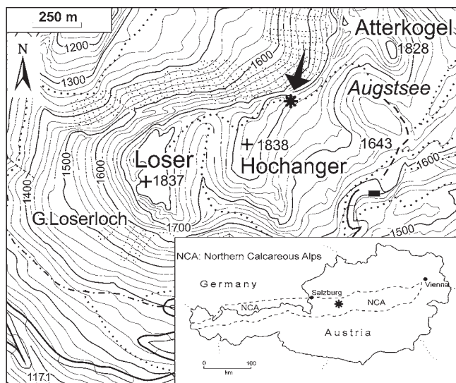
Text-Fig. 4. Topographic map of the Loser area. The sample containing the holotype of Rivularia? loseri n. sp. is marked with an asterisk.
