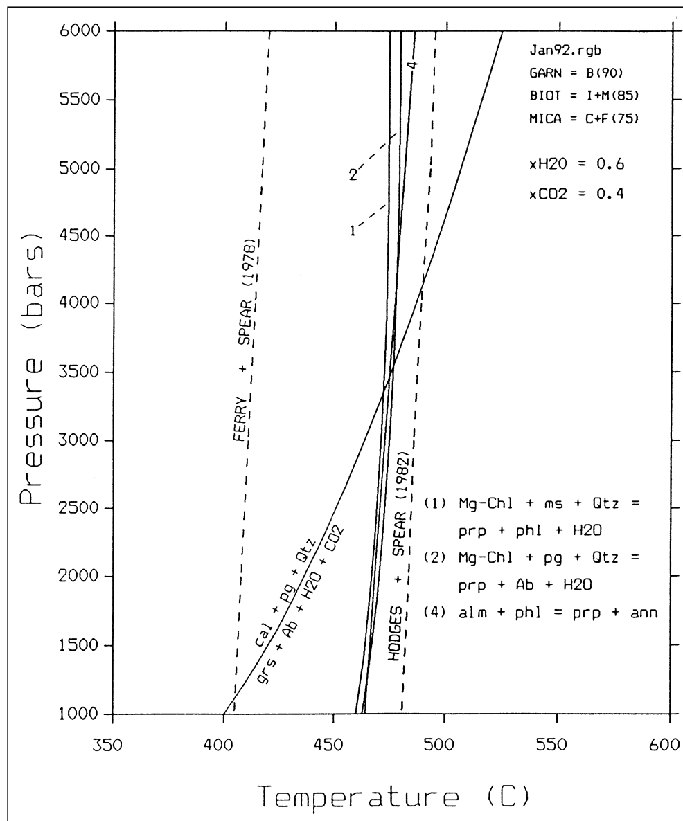
Text-Fig. 9. P-T diagram of the sample DB-27 (discussed in the text). Symbols of minerals after KRETZ (1983).
