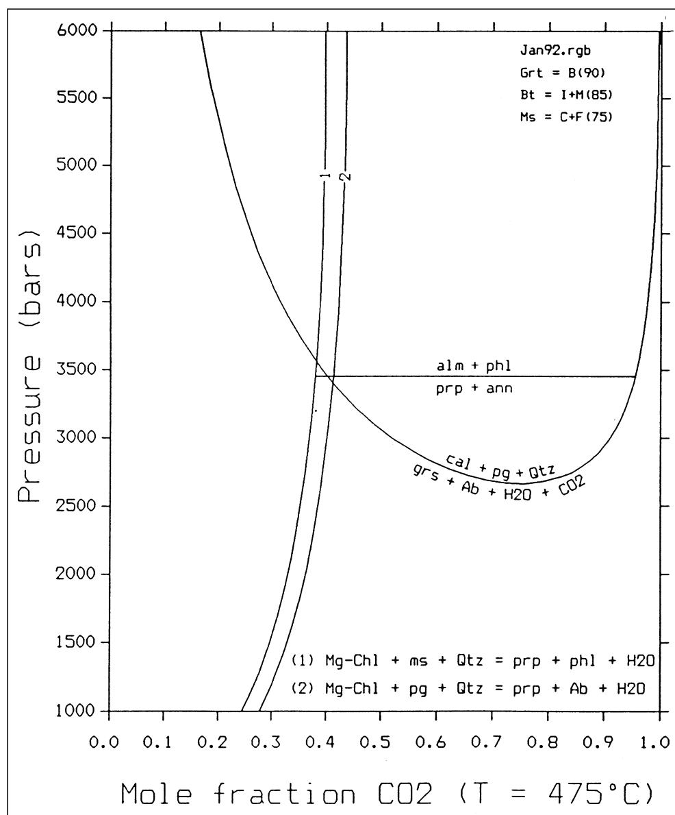
Text-Fig. 10. P- X_{\text{CO}_2} diagram of the sample DB-27 (discussed in the text). Symbols of minerals after KRETZ (1983).
