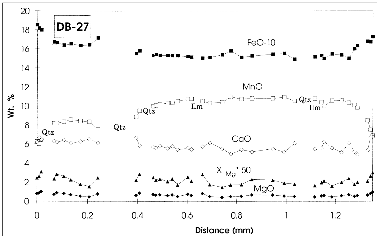
Text-Fig. 7. Cross profile through a garnet porphyroblast elongated in s. Despite of the flat element distribution a slightly bell-shaped Mn profile with compensating bowl-shaped Fe profile is recognized.
