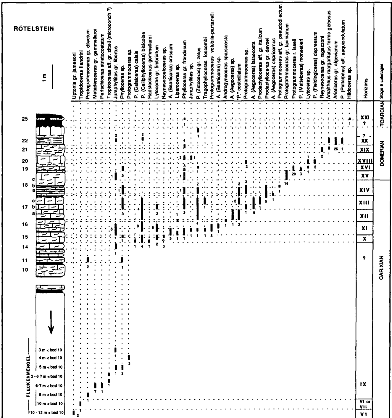
Text-Fig. 8. Rötelsstein. Lithological profile and ammonite ranges.
