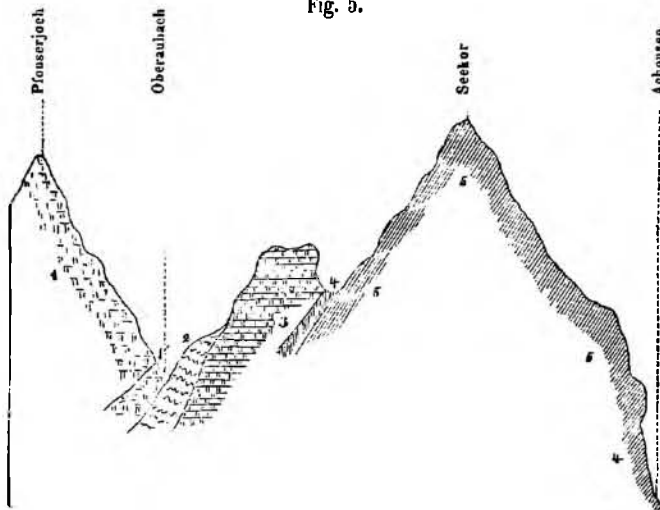
1. Aptychen-Kalk. 1'. Rother Hornstein. 2. Adnether-Schichten. 3. Lithodendron-Kalk. 4. Gervillien-Schichten. 5. Dolomit.
