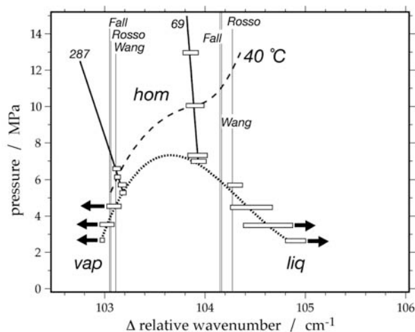
Fig. 3. Peak position difference of the Fermi double of \text{CO}_2 as a function of pressure, density (in molar volume: 69 and 287) and temperature ( 40 \text{ }^\circ\text{C} ).
