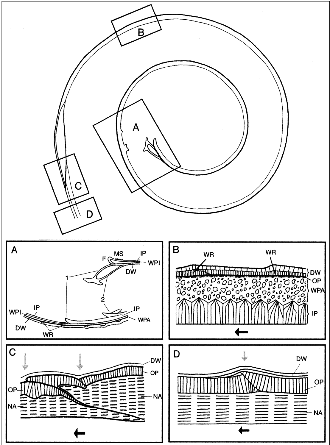
Text-Fig. 3. Median cross-section through the embryonic shell of a goniatite. The letters indicate the locations of the close-ups shown below.
