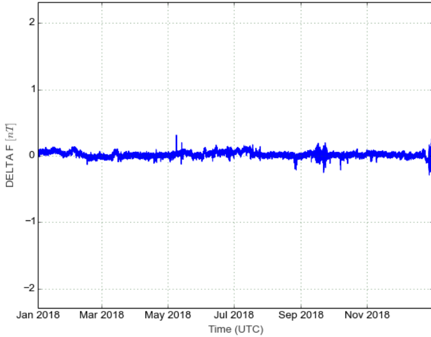
Figure 4.3 Delta F values between the scalar magnetometer and the field strength calculated from the baseline corrected vectorial data set. The scale of the figure is related to the INTERMAGNET 5 nT criteria.
