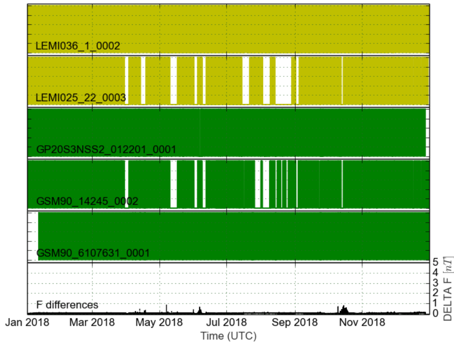
Figure 4.5 Contributions of each sensor for the analysis of 2018. Yellow shaded regions indicate time ranges of respective variometer data, green shaded regions mark scalar data which has been averaged for the composite one-minute record. The lowermost plot depicts the average difference between all scalar data.
