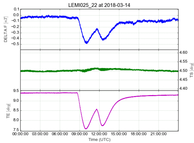
Figure 5.2 Delta F values of the definitive data from the secondary variometer LEMI025 (SN: 22) relative to the primary F sensor, as well as temperatures of the variometers sensor (Ts) and its electronics (Te) for a single day when the cabinet containing the electronics was opened. The effect on delta F is clearly visible.
