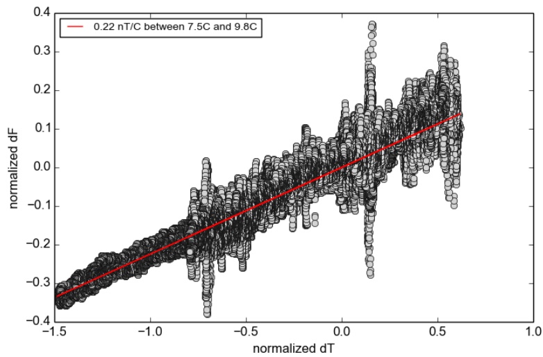
Figure 5.3 Cumulative plot of normalized temperature variations of the sensor electronics versus normalized delta F variations for altogether 5 days when the electronics cabinet was opened. Sensor temperature variations are negligible.
