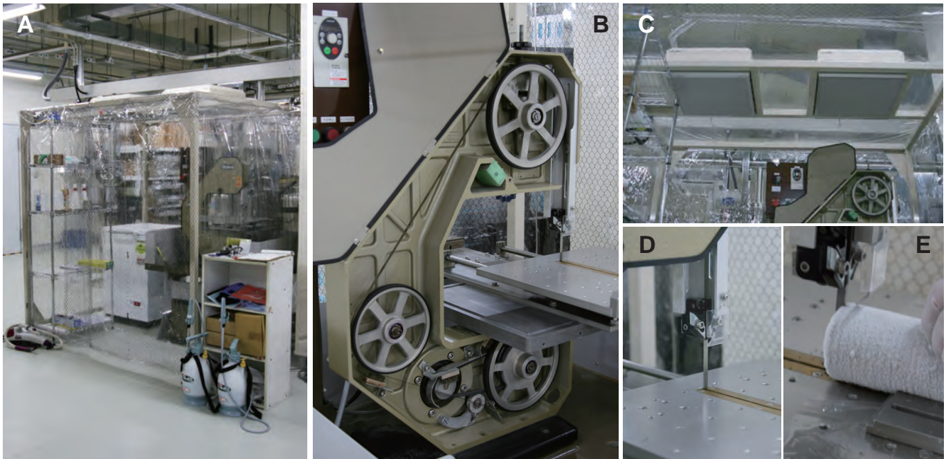
Figure 2. [A] Overview of the electric band saw system for microbiological frozen core. Motor-driven electric band saw machine [B] and -50^{\circ}\text{C} freezer is deployed in a clean booth equipped with two HEPA-filter units [C]. Diamond-tipped band saw cuts frozen core samples under clean conditions [D, E].
