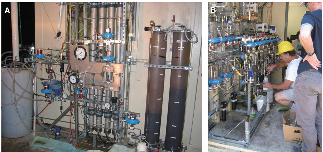
Figure 2. The Frio Brine Pilot surface sampling systems: [A] Four 13 L high pressure sample vessels mounted in sliding sleeves and resting on strain gauges to measure fluid density. [B] Computer-operated valve manifolds used to operate the U-tube samplers.
