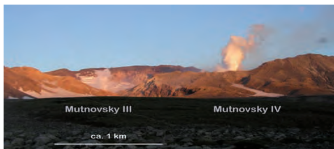
Figure 2. Mutnovsky Volcano from the west. The Crater Glacier and the hydrothermal plume of Mutnovsky III crater is visible through the breach formed by the Volcannaya River in Dangerous Ravine left of center. The larger plume from the Active Crater of Mutnovsky IV rises to the right. Width of the field of view is approximately 3 km (photo by J. Eichelberger).
