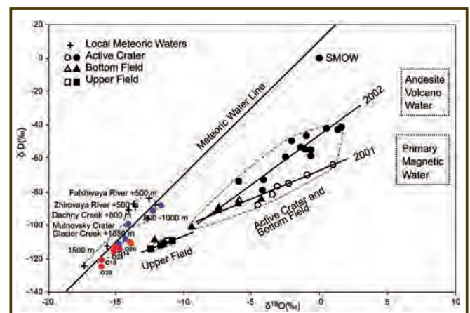
Figure 5. Integrated δD vs δ 18 O data of the Mutnovsky geothermal field (red circles - production wells, blue circles - meteoric waters; Kiryukhin et al., 1998; 2002) and Mutnovsky crater fumaroles (Zelensky et al., 2002).
