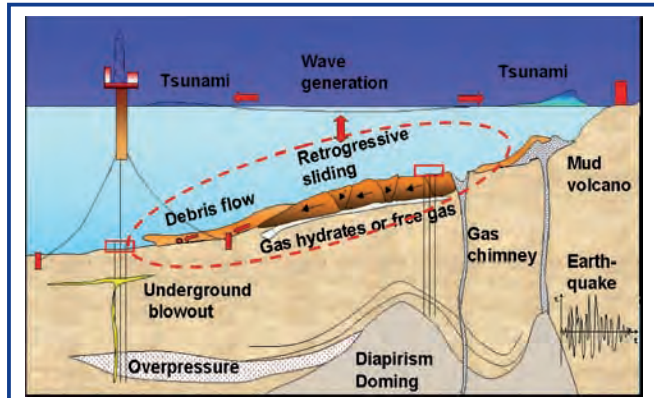
Figure 4. Summary of slope processes that may contribute to failure, generating landslides, debris flows, and tsunami (from Camerlenghi et al., (2007), courtesy Norwegian Geotechnical Institute (NGI) and the International Centre for Geohazards (ICG).
