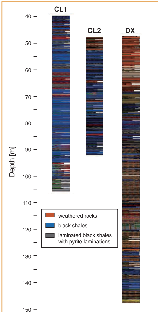
Figure 4. Integrated stratigraphic columns for CL1, CL2, and DX in DXCL-DP based on fine-scale visual inspection of the drillcores. Note that the upper ~40-m sections of cores (highly-weathered by recent oxidation) were not sampled.
