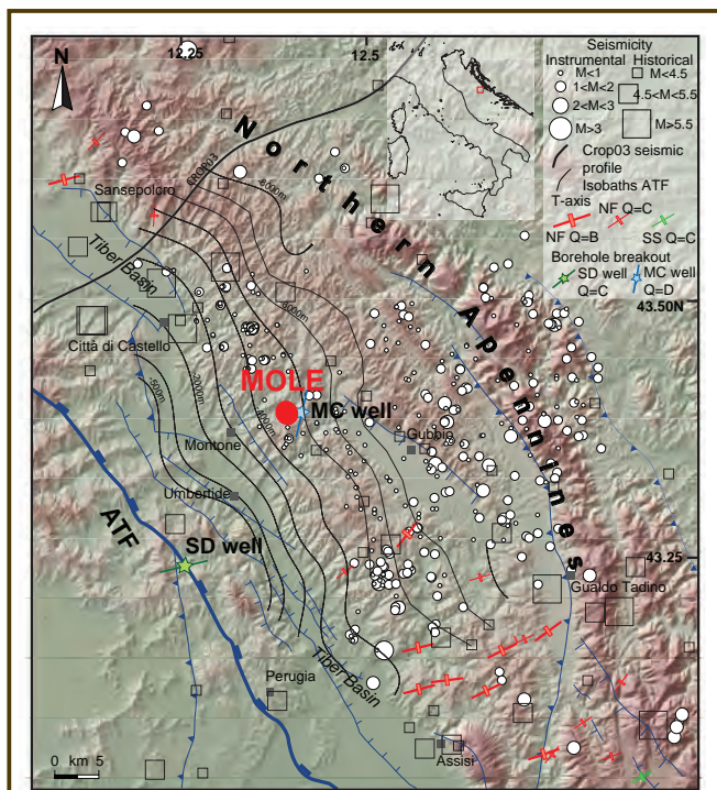
Figure 5. Digital Elevation Model around the planned MOLE borehole (red circle) showing the seismicity (instrumental from Chiaraluze et al., 2007 and historical from Boschi et al., 2000), T-axes from focal mechanisms (Montone et al., 2004), breakout data (Mariucci et al., 2008) and Alto Tiberina Fault isobaths (Mirabella, 2002).
