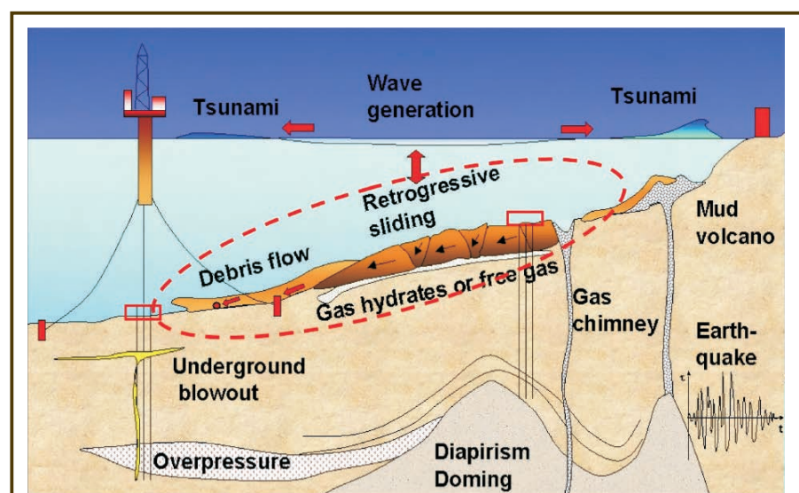
Figure 1. Offshore geohazards. Submarine slides generated by human activity are recognized as submarine geohazards for first party seabed structures and for third party (population) because of their potential to generate tsunamis. Submarine slides are known to occur also as a consequence of the natural evolution of continental margins.
