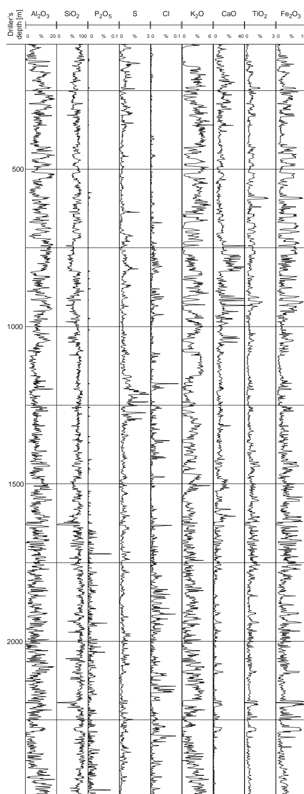
Figure 2. Preliminary chemical data of major elements produced by the new instrument of the full length of the COSC-1 drill core, scanned with 0.1 m resolution.
