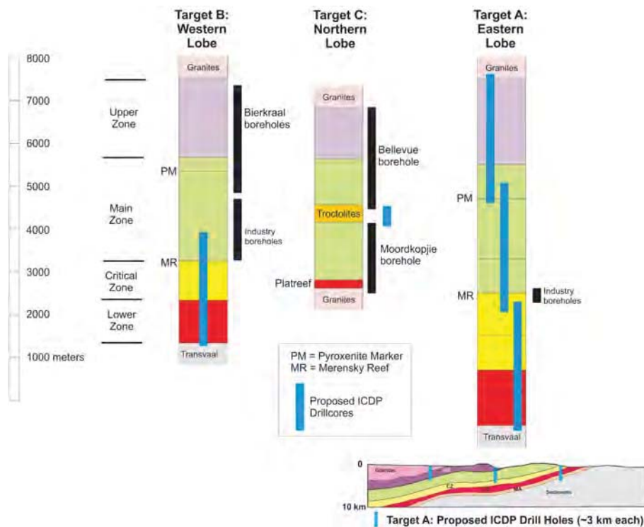
Figure 3. Schematic stratigraphic sections of the Bushveld lobes illustrate ICDP targets A, B and C. The cross section of the eastern lobe (right) explains the staggered-hole concept for target A (see text).
