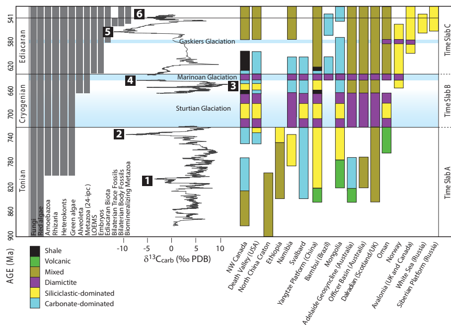
Figure 2. Schematic timeline showing major evolutionary events, a composited \delta^{13}C curve with numbered isotope anomalies (1 – Bitter Springs; 2 – Islay; 3 – Keele Peak; 4 – Trezona; 5 – Shuram; 6 – BASE) and an approximation of the stratigraphic distribution and dominant lithology type for a number of key Neoproterozoic successions that occur worldwide. Time slabs identified for drilling are shown on the right.
