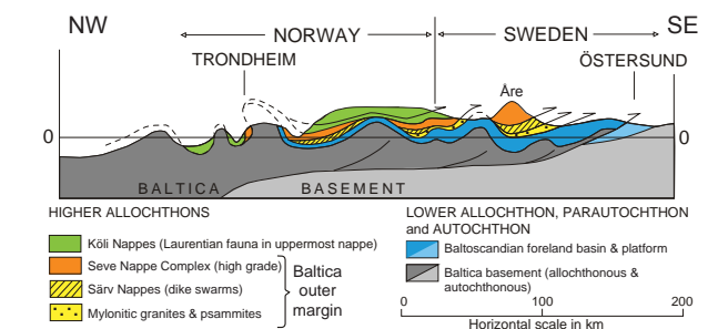
Figure 2. Tectonostratigraphic map of the Scandinavian Caledonides and sketch section along the geotraverse from Östersund to the Norwegian coast. Modified from Gee et al. (2010).
