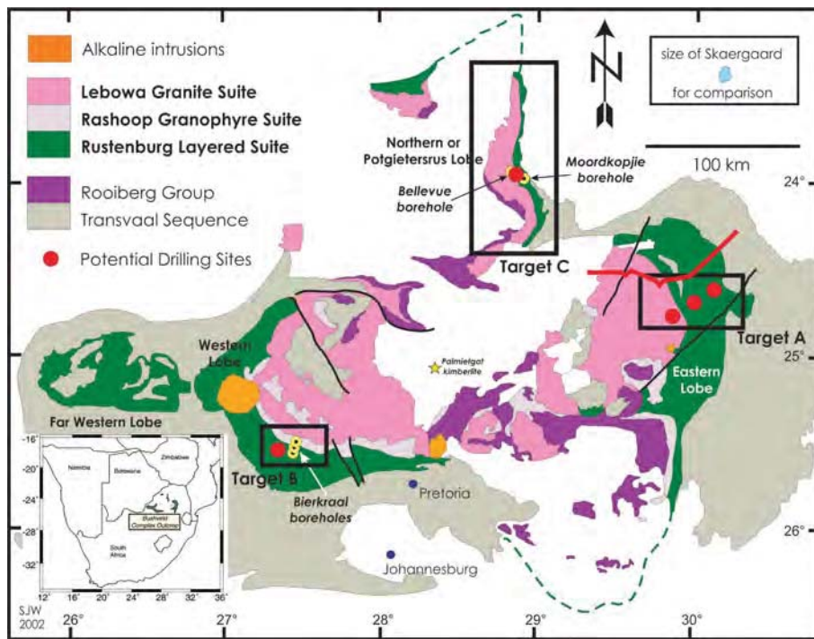
Figure 1. A simplified map of the Bushveld Complex with location of existing boreholes (yellow) and the potential ICDP sites in the western, northern and eastern lobes (red dots in boxes). The inset in upper right shows the size of the iconic Skaergaard layered intrusion for comparison. The thick red line above target A is a reflection seismic line of the Council for Geoscience. The Palmietgat kimberlite in the centre of the complex (star) contains Bushveld xenoliths, confirming geophysical evidence for a continuity of E and W lobes (see text).
