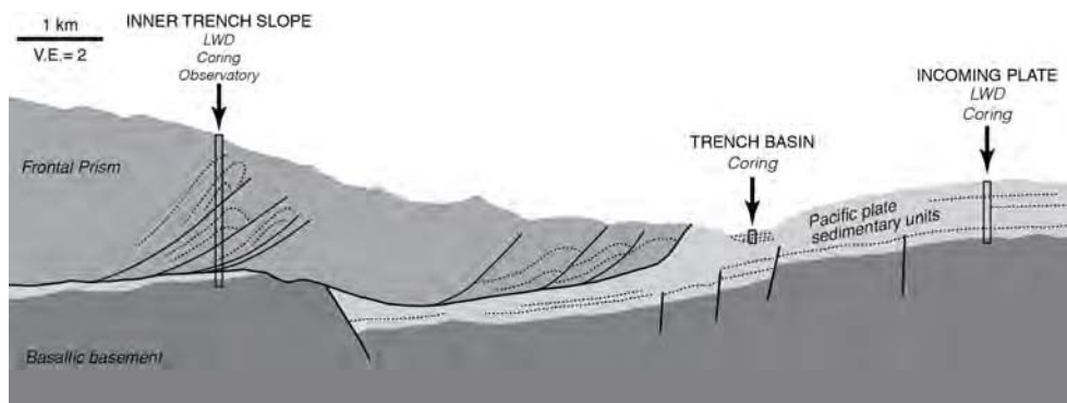
Figure 2. Schematic section through the frontal prism, trench and incoming section showing the framework for the two proposed trench normal transects, locations of the holes and list of target data for each hole (dashed lines represent possible bedding attitudes; solid lines are possible faults; structure based on Nakamura et al., 2013).
