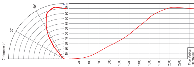
Figure 8. The COSC-1 drill hole deviation, seen from above (with azimuth) and plotted vs. depth: 10 × horizontal exaggeration.
