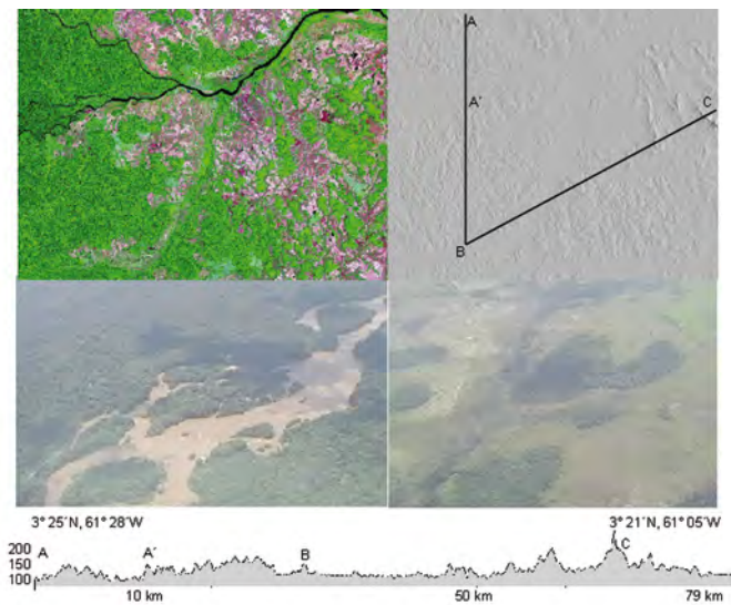
Fig. 8: "A-A'" – Uraricoera River (left photo); B – Grande River; C – Serra do Taboão. Region of the endemic lizards Gymnophthalmus vanzoi and G. leucomystax (family Gymnophthalmidae ). Forest and lavrado contact, with small patches of forest (right photo). Transition of denudational and aggradational relief, with isolated hills, drained by a not well development fluvial plain.
