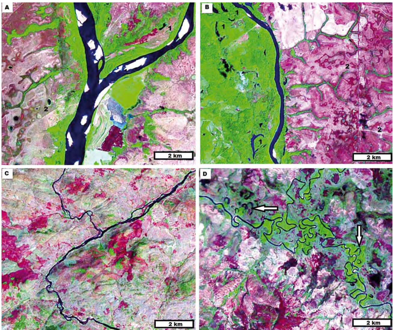
Fig. 6: "A-B" – fluvial plains, lowlands (03°01'N, 60°29'W and 02°36'N, 60°54'W); "C-D" – fluvial plains, highlands (04°17'N, 60°32'W and 04°56'N, 61°14'W). 1 – abandoned chanel lakes of flood plain; 2 – Lakes of flat plain. A – Mouth of the Tacutu River in the Branco River; B – Mucajaí River; C – Cotingo River with structural control, non flood plain; D – meandriform river developed at structural control, small flood plain with lacustrine systems (oxbows lakes).
