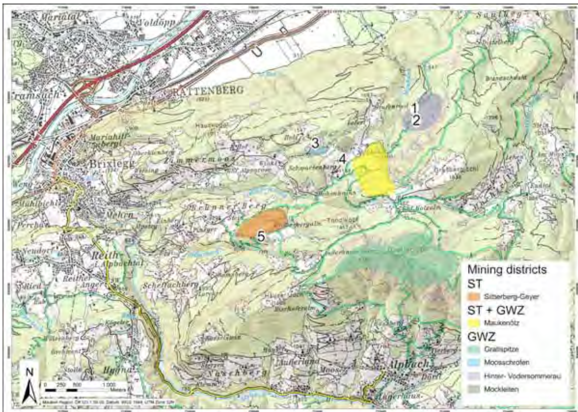
Fig. 4 One of the most outstanding examples of an ore district in the ST is the Geyer-Silberberg mining district. This mining area is located to the north of the Grattspitze-Hauser Joch ridge. The southernmost ore zone of the Geyer-Silberberg district is the Geyerköpfl. The second important mining area in Triassic rocks in the Mauken Area is Maukenözt.
