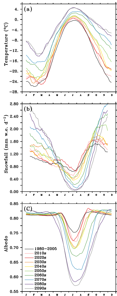
Figure 9. (a) Mean annual cycle of TAS ( ^{\circ}\text{C} , 30-day running mean) over the permanent ice covered area for the listed decades. The 1980–2005 mean is given in black as comparison. (b) Same as (a) but for the snowfall ( \text{mm w.e. d}^{-1} ). As the daily variability of precipitation is very high, we have applied here a 60-day running mean instead of 30 days (like in Figs. 8 and 9a and c) in order to make the figure more clear. (c) Same as (a) but for the albedo.
