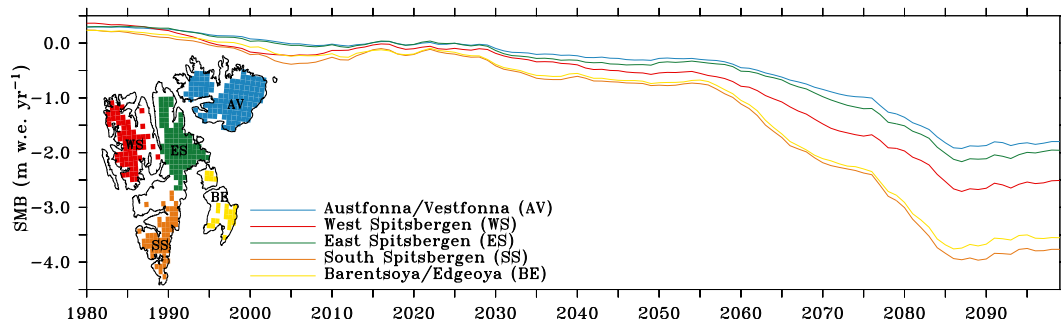
Figure 3. SMB 10-year running mean ( \text{m w.e. yr}^{-1} ) for five different regions (Austfonna and Vestfonna, west Spitsbergen, east Spitsbergen, south Spitsbergen and Barentsøya and Edgeøya) as simulated by MAR forced by the MIROC5-based historical scenario over 1980–2005 and RCP8.5 afterwards. The units are in \text{m w.e. yr}^{-1} (rather than \text{Gt yr}^{-1} ) to be independent of the different areas of the regions. The permanent ice mask of each region defined for the regional evolution is shown in the inset.
