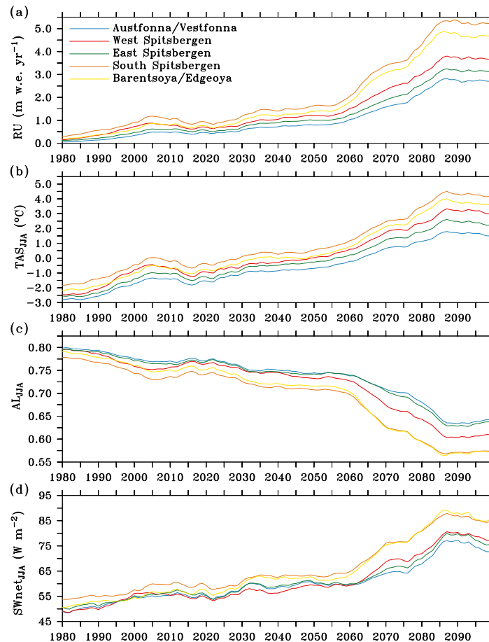
Figure 4. (a) 10-year running mean of the meltwater runoff (RU, \text{m w.e. yr}^{-1} ) over 1980–2099 for the five regions shown in Fig. 3. (b) Same as (a) but for the near-surface JJA temperature ( \text{TAS}_{\text{JJA}} , ^{\circ}\text{C} ). (c) Same as (a) but for the JJA albedo ( \text{AL}_{\text{JJA}} ). (d) Same as (a) but for the JJA net solar radiation absorbed by the surface ( \text{SWnet}_{\text{JJA}} , \text{W m}^{-2} ).
