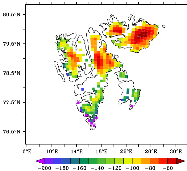
Figure 5. Projected cumulated anomaly of SMB changes (m.w.e.) over the 21st century. The SMB anomaly is the difference with the 1980–2005 mean and has been summed over 2000–2100.
