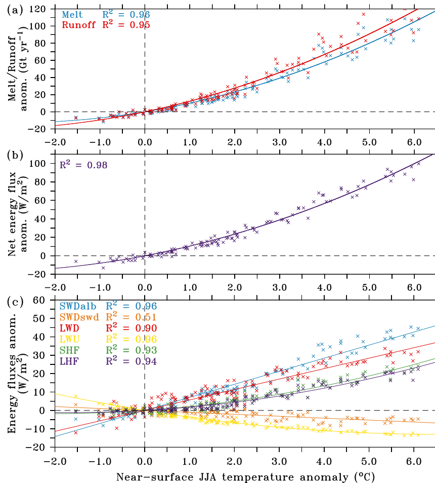
Figure 10. (a) Melt and runoff anomalies ( \text{Gt yr}^{-1} ) vs. \text{TAS}_{\text{JJA}} anomaly ( ^{\circ}\text{C} ). The anomalies are differences with respect to the 1980–2005 mean. (b) Same as (a) but for the JJA net energy flux at the surface ( \text{W m}^{-2} ). (c) Same as (a) but for the JJA energy balance components. The solid lines are quadratic regression curves.
