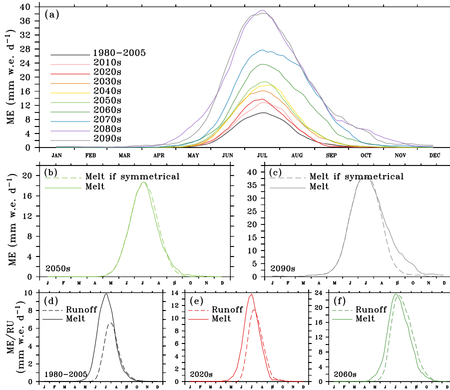
Figure 8. (a) Mean annual cycle of the surface melt (mm w.e. d -1 , 30-day running mean) for the listed decades. The 1980–2005 mean is shown in black as comparison. (b) Annual cycle of the surface melt in the 2050s (solid line) as well as, in dashed lines, the cycle if it were symmetrical with respect to its maximum. (c) Same as (b) but for the 2090s. (d) Mean annual cycle of melt (solid line) and runoff (dashed line) (mm w.e. d -1 ) during the 1980–2005 period. (e) Same as (d) in the 2020s. (f) Same as (d) in the 2060s.
