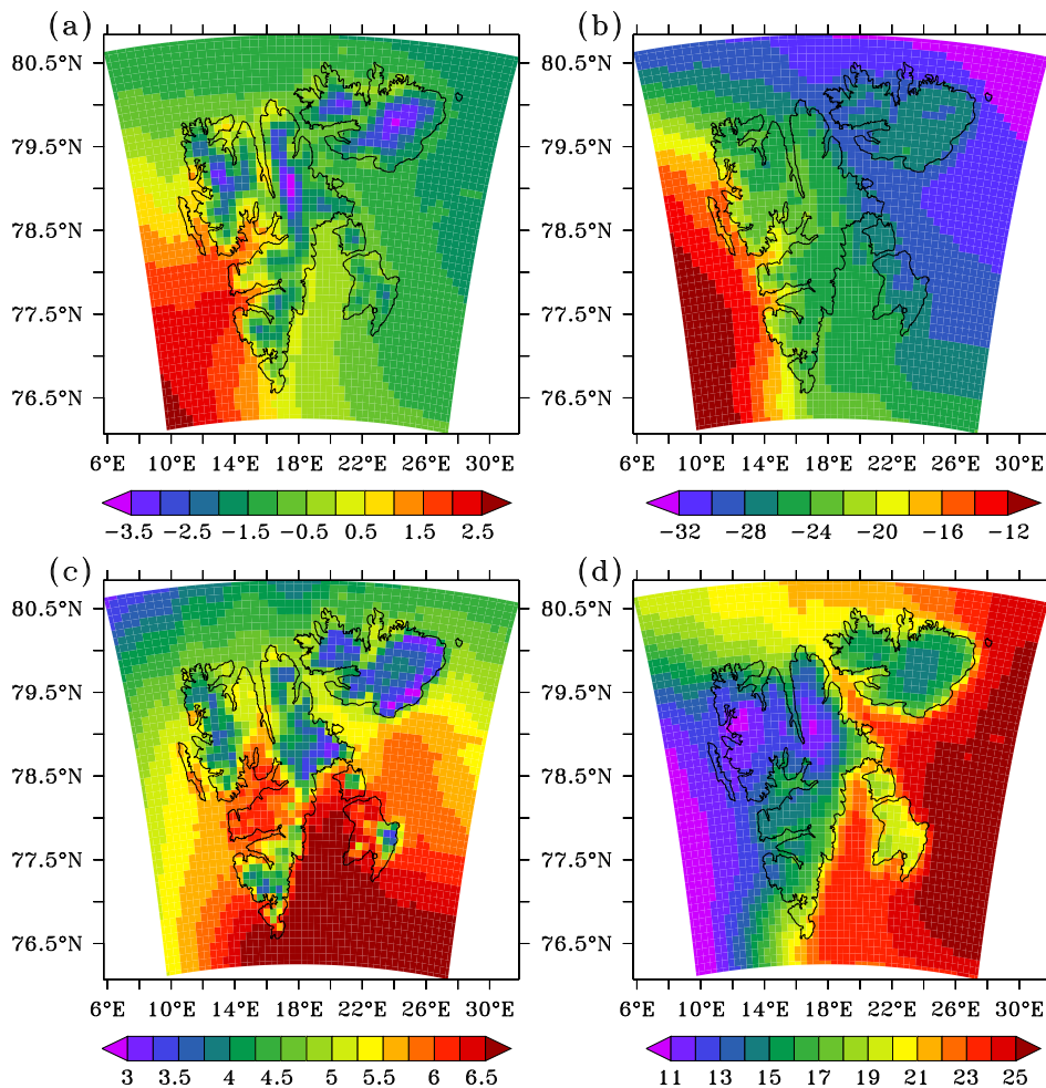
Figure 7. (a) 1980–2005 mean summer (JJA) near-surface temperature ( ^{\circ}\text{C} ). (b) Same as (a) but for winter (DJF). (c) 2070–2099 mean summer (JJA) near-surface temperature anomaly ( ^{\circ}\text{C} ) with respect to the 1980–2005 mean. (d) Same as (c) but for winter (DJF).
