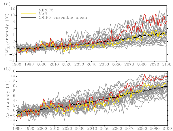
Figure 1. (a) 1980–2100 evolution of the JJA near-surface temperature (TAS JJA , °C) anomaly over Svalbard with respect to the 1980–2005 mean simulated by MIROC5 (red curve), the CMIP5 GCMs (grey curves), the ensemble mean (black curve) and MAR forced by MIROC5 under the RCP8.5 scenario (yellow curve). (b) Same as (a) but for the annual near-surface temperature.
