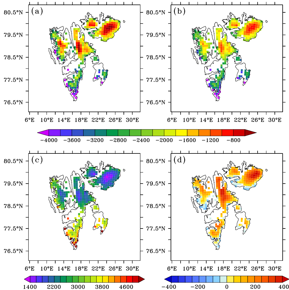
Figure 2. (a) 2070–2099 mean SMB ( \text{mm w.e. yr}^{-1} ) as simulated by MAR forced by the MIROC5-based RCP8.5 scenario. (b) Difference between (a) and the 1980–2005 mean shown in Fig. 14 in Lang et al. (2015). (c) Same as (b) but for runoff. (d) Same as (b) but for precipitation.
