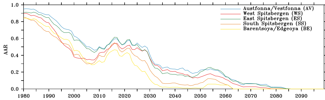
Figure 6. 10-year running mean of the accumulation area ratio (AAR) over 1980–2099 for the five regions shown in Fig. 3. AAR represents the ratio of the area of the accumulation zone of a region compared to the total area of the region, i.e. the proportion of a region that is in the accumulation area.
