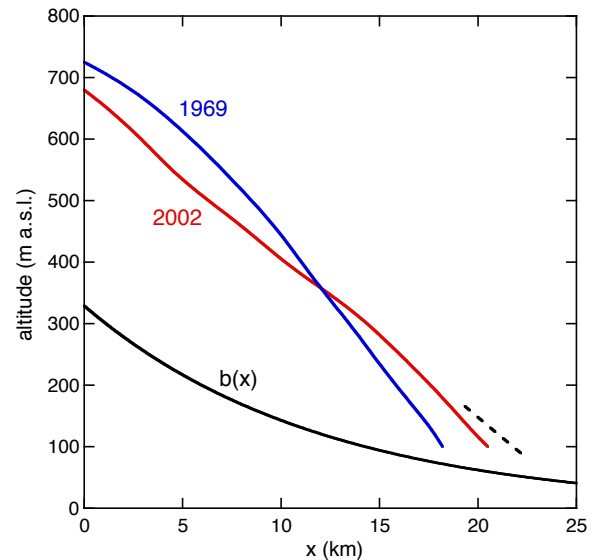
Figure 4. Altitude profiles along the central flow line of Abrahamsenbreen derived from topographic maps. The surge took place around 1978. The dashed line indicates a possible maximum extension of the glacier immediately after the surge. The reference bed profile is shown as b(x) .
