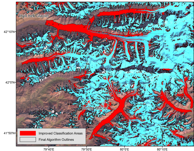
Figure 3. Final algorithm outlines (black) with areas classified in addition to the clean-ice delineation in red. Landsat OLI image captured on 25 September 2013 as background.
