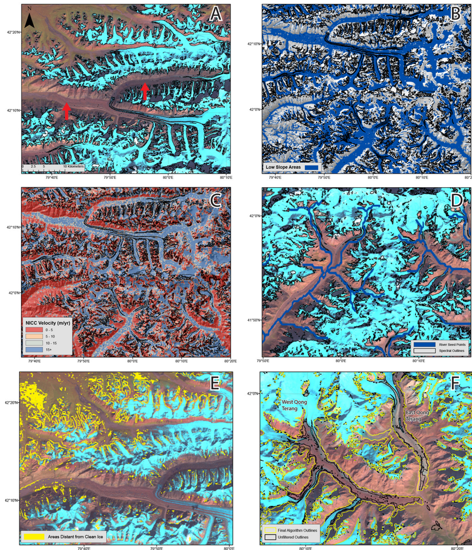
Figure 2. (a) Characteristic example of a debris-covered glacier tongue (Inylchek Glacier). Spectrally delineated glacier outlines (black), over Landsat bands B7/B5/B3 (R/G/B), from image LC81470312013268LGN00, with poorly mapped debris-covered tongues (red arrows). (b) Blue areas show “potential debris areas”, as delineated by slopes between 1–24°, with elevations below ~2500 m removed, SRTM hillshade underneath, clean-ice outlines overlain in black. (c) Example of a glacier velocity surface, generated using normalized image cross-correlation (NICC). Areas in red are slow-moving areas and represent stable ground, clean-ice outlines overlain in black. (d) Example of distance-weighting seed areas used to remove pixels from the “potential debris areas” which are distant from either a river valley or classified glacier ice. Rivers in blue, clean-ice outlines overlain in black. (e) Areas removed by second distance-weighting step (yellow). (f) Impacts of statistical filtering on glacier outlines, with areas in black removed during the filtering process. East and west Qong Terang glaciers.
