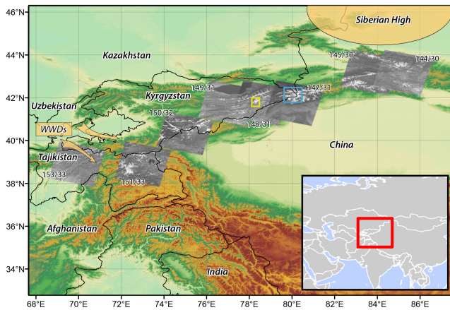
Figure 1. Greater study area of the Tien Shan, showing SRTM v4.1 topography (Jarvis et al., 2008) and location of eight Landsat image footprints (grayscale) used in the study, along with their Path/Row combinations. Blue box delineates Figs. 2, 3 and 7, yellow box delineates Fig. 8. Winter westerly disturbances and Siberian High highlighted in orange.
