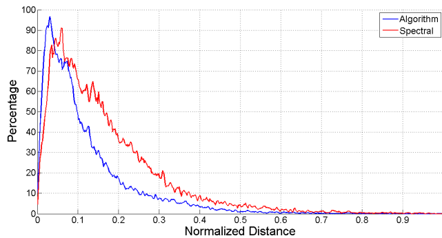
Figure 6. Vertex distance distributions for algorithm (blue) and spectral (red) vertices, as compared to a manual control data set, normalized to the maximum distance.
