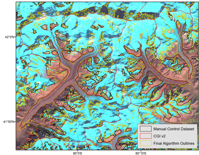
Figure 7. Algorithm outlines (yellow) compared to the control data set (black) and the CGI v2 (red) illustrate high fidelity in overall debris-tongue length between the three data sets, although the algorithm outlines exhibit noise along the edges of debris tongues.
