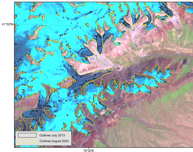
Figure 8. Algorithm outlines for July 2013 (black) and algorithm outlines for August 2002 (yellow), showing small retreats in glacier areas, particularly at the debris tongues. Vicinity of the Akshiirak glacierized massif, central Tien Shan.
