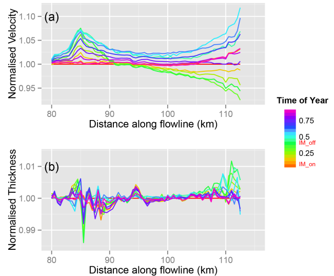
Figure 8. Plots showing velocity (a) and thickness (b) perturbations through a single calendar year. Line colour indicates time of year. Velocity and thickness have been normalised against their 1 January values.
