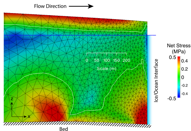
Figure 3. The terminus of the flow line mesh of Store Glacier. White line indicates the net stress ( \sigma_n ) zero contour for both surface and basal crevasses. Net stress (MPa) is > 0 where crevasses exist and < 0 in solid and unfractured ice. Calving occurs in the model when the surface and basal zero contours meet. The blue line indicates sea level.
