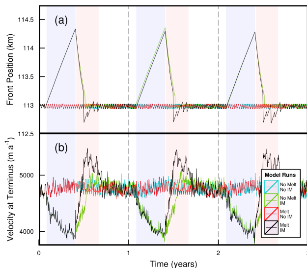
Figure 6. Plots showing changes in calving terminus position (a) and velocity (b) during a 3-year period within a 40-year-long stable simulation, with coloured solid lines illustrating the effect of four different combinations of melting and ice mélange perturbation. Blue and red shading indicates mélange and melt season, respectively.
