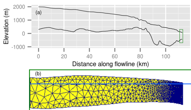
Figure 2. (a) Surface and basal geometry of central flow line used in this study. (b) Model mesh of region outlined by green box in (a). The blue line represents sea level.
