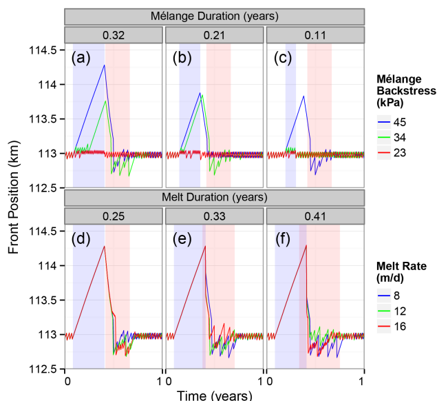
Figure 9. Plots showing terminus position through 1 year for varying mélangé season duration (a–c) and melt season duration (d–f). Durations of mélangé and melt season are indicated by blue and red shading, respectively. Line colour indicates varying magnitude of melt rate and mélangé backstress. The blue line in panels (a) and (d) represent the baseline model from experiment 1 (Fig. 6). Changing panels and line colours indicate perturbations under progressively warmer climate scenarios.
