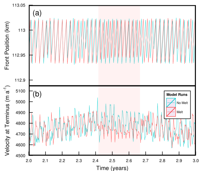
Figure 5. Plots showing variations in terminus position (a) and velocity (b) over the course of a year for the baseline model run (blue line) and a run with submarine melting applied (red line). Red shading indicates melt season. The saw-toothed pattern in both panels is a result of calving.
