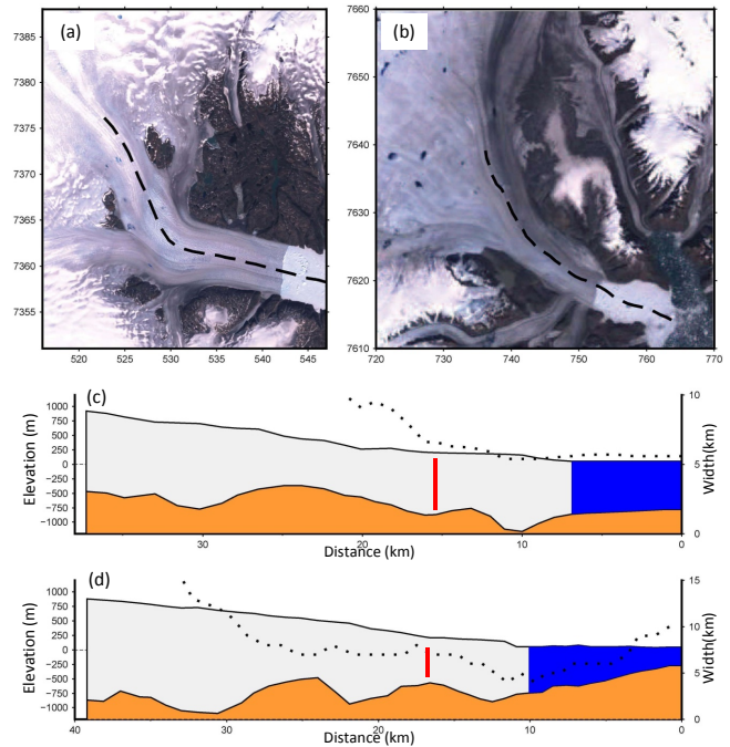
Figure 11. (a) : Landsat7 ETM+ “true color” image of Helheim Glacier from 2 August 2001; (b) : Landsat7 ETM+ “true color” image of Kangerdlugssuaq Glacier from 6 August 1999; (c) : Bedrock and ice surface profiles along the dashed line shown in (a) . The dotted curve represents width of Helheim Glacier along the same profile. The vertical red line denotes minimum retreat of the Helheim Glacier (which occurred in 2005, see Fig. 8). (d) : Same as (c) but for Kangerdlugssuaq Glacier. The minimum retreat of the Kangerdlugssuaq Glacier occurred in 2012 (see Fig. 9). Bed data is obtained from Bamber et al. (2013).
