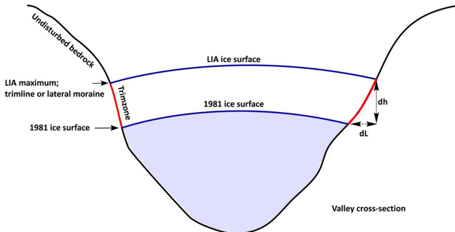
Figure 6. Sketch of outlet glacier perpendicular to the flow direction. Points are placed at the trimline or lateral moraine marking the LIA_{max} position and at the 1981 ice surface. The vertical difference ( dh ) is the thinning at each sample location.
