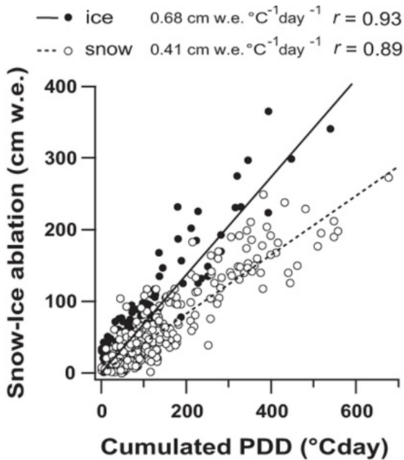
Fig. 10. Measured ablation at stake 4 for snow and ice as a function of the cumulated positive degree day calculated from Lyon with a vertical lapse rate of 6.25 \text{ } ^\circ\text{C km}^{-1} .
