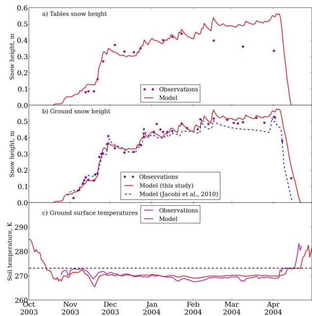
Fig. 6. Simulations of the seasonal evolution of snowpack height with Crocus. (a) On tables; (b) on the ground. Experimental data and the previous work of Jacobi et al. (2010) are also shown for comparison. Panel (c) displays the simulated and observed ground surface temperature.
