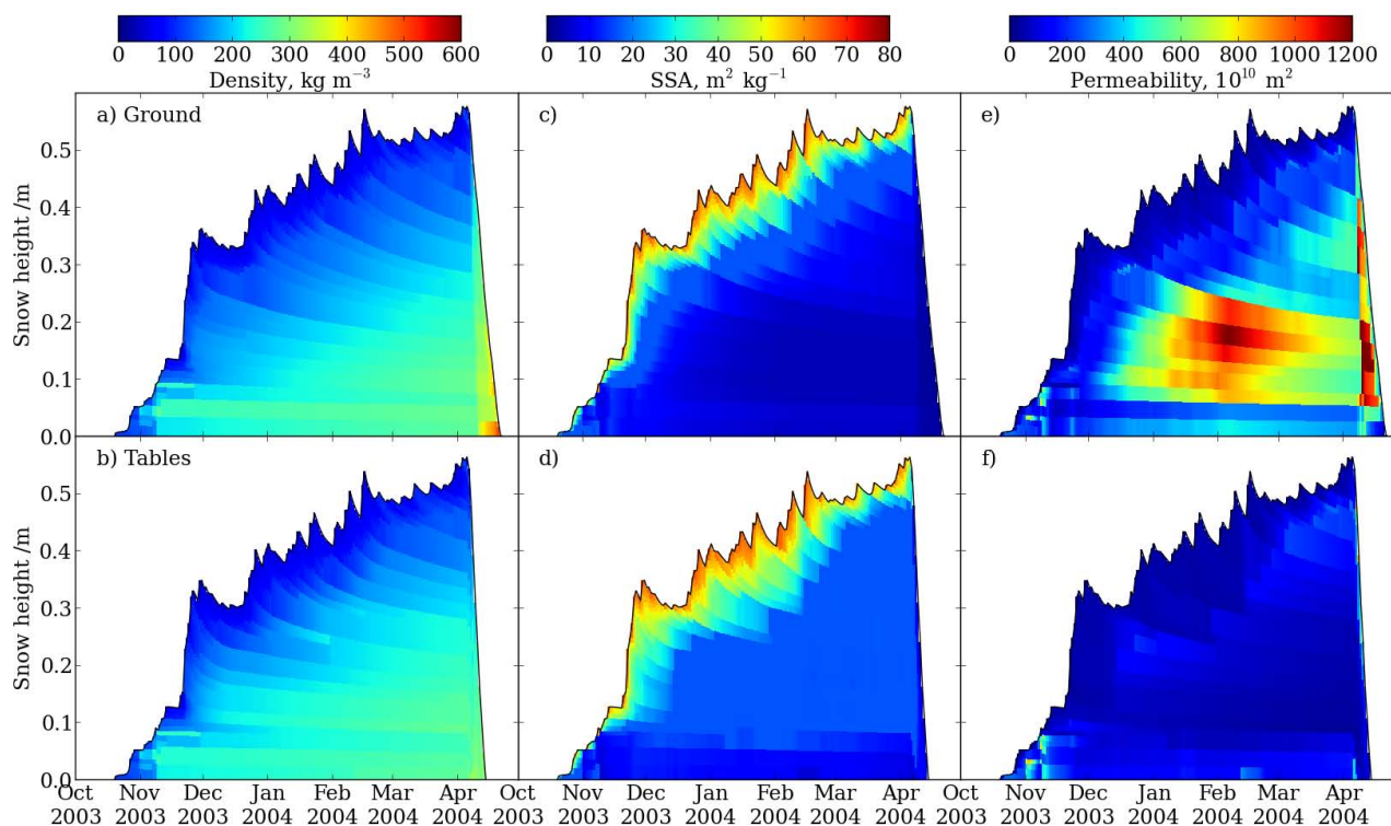
Fig. 8. Simulations of the vertical profiles of density (a, b), SSA (c, d) and permeability (e, f) on the ground (a, c, e) and on tables (b, d, f) simulated using the snowpack model Crocus, over the whole season.
