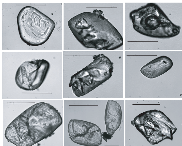
Fig. 3. Examples of ikaite crystals found in the sea ice. Scale bar is 100 µm.
