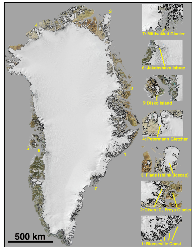
Fig. 1. Greenland ice outlines, simplified from outlines to be reported by Citterio et al. (2012), overlain on a 250 m MODIS mosaic of Greenland made by Paul Morin. See Supplement Fig. S1 for a full resolution, unannotated version and further details. Insets highlight glaciers and icecaps discussed in the text.
