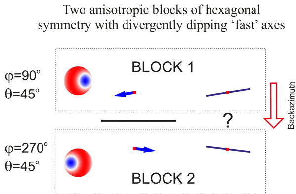
Figure 4. Fast S polarizations evaluated for synthetics propagating through two blocks with divergently inclined fast symmetry axes. The “arrow style” of presentation shows the domain boundary while the standard approach (azimuthal) does not.
