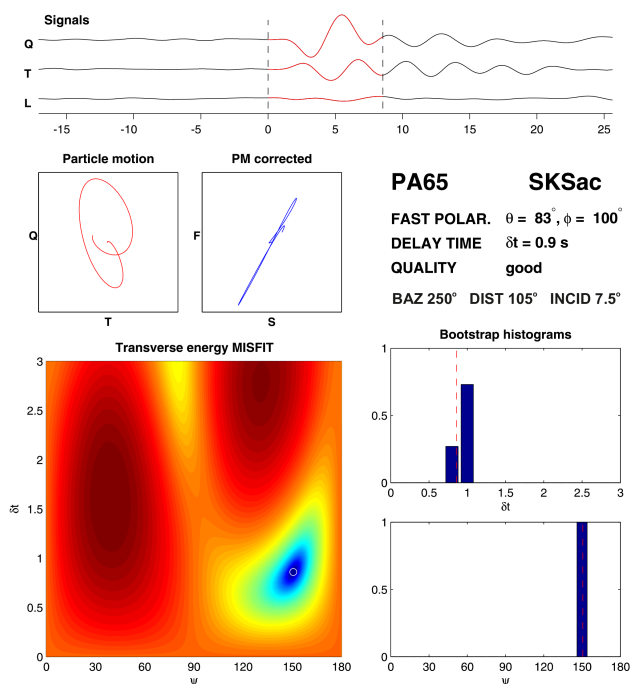
Figure 3. Example of evaluation of SKSac phase splitting at station PA65 in the central part of the PASSEQ array (see Fig. 2) for an earthquake in the Chile–Argentina border region: 2006-08-25_00:44, 24.34° S 67.01° W, 185 km deep, 5.8 Mw. Epicentral distance to the station is 105.2°, back-azimuth 250.0° and incidence angle 7.5°. For more details of the method see Vecsey et al. (2008).
