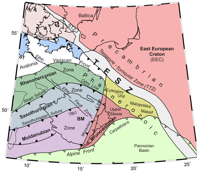
Figure 1. Simplified tectonic sketch of the Trans-European Suture Zone (TESZ) and adjacent areas according to Pharaoh (1999). STZ stands for the Sorgenfrei-Tornquist Zone, TBU for the Teplá-Barrandian Unit included in the Moldanubian Zone of the Bohemian Massif (BM).
