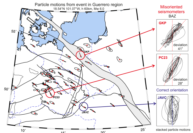
Figure 5. Horizontal shear-wave particle motion (PM) across the PASSEQ array for an event from the NW (left), located in Guerrero region, documenting incorrect northward orientation of seismometers at stations GKP and PC23. PMs rotated to the back azimuths and stacked for all events evaluated at stations PC23 and GKP with misoriented seismometers, and correctly aligned seismometer at JAVC (right). Only sufficiently large errors ( \sim > 10^\circ ) in seismometer misorientation can be revealed by this method. Smaller deviations of the PM can be caused by a weak anisotropy in the upper mantle.
