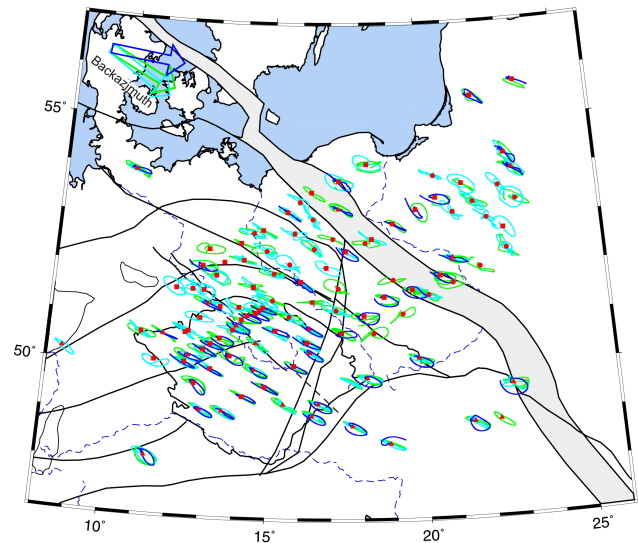
Figure 11. PMs for the same events from the NW as in Fig. 10.
