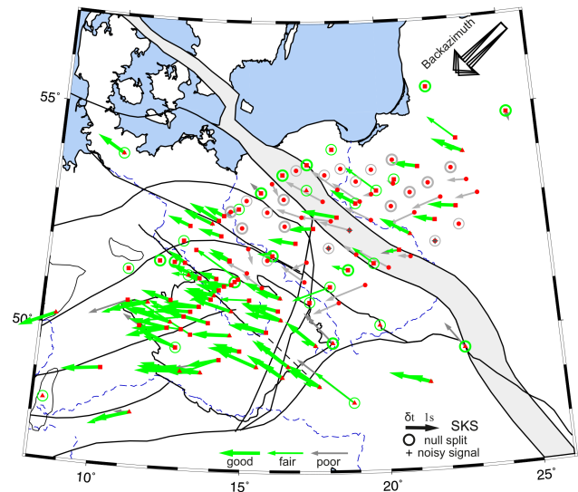
Figure 8. Azimuths \varphi of the fast shear-wave polarizations and the split-delay times \delta t evaluated for three events from the NE back azimuths. Anisotropic signal dominates in the Bohemian Massif, null splits or small provinces with coherent polarizations exist west and north of the Bohemian Massif. Complementary measurements at stations equipped with 2–3 s seismometers are shown in light-grey colour.
