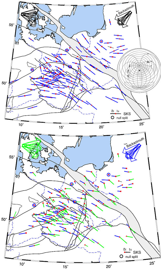
Figure 6. Shear-wave splitting presented in a standard way, i.e. the fast shear-wave polarization azimuths (Supplement Table S1) as bars with length proportional to the split delay time: (a) averages calculated from all measurements regardless of wave back azimuth and (b) averages calculated separately for waves arriving from the west and from the northeast. Inset shows epicentre distribution of 15 events used in this study relative to the PASSEQ array (star).
