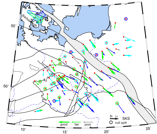
Figure 10. Azimuth \varphi of the fast shear-wave polarizations and delay times \delta t evaluated for four events from the NW back azimuths. Green arrows represent results stacked for two events. Nulls or near-null splitting prevail in the BM and in the western part of the array, whereas stations east of the Moravian Line show strong anisotropic signal for this back-azimuth interval.
