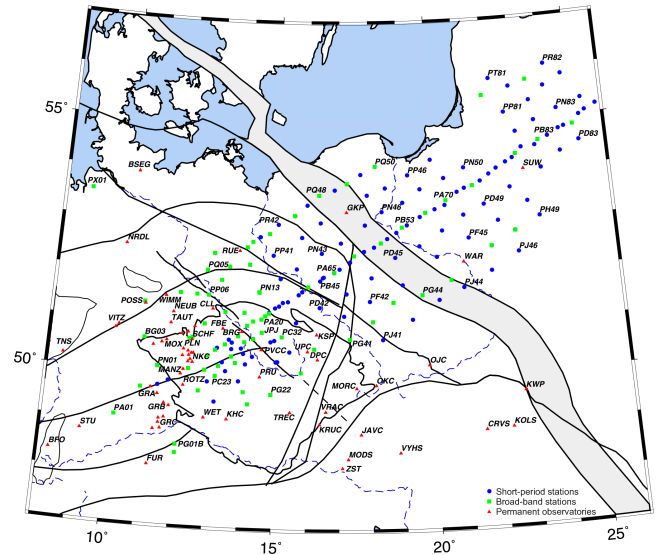
Figure 2. Seismic stations of the passive experiment PASSEQ (2006–2008) designed to study upper mantle structure of the TESZ. Labels are assigned to some of stations for easier orientation.
