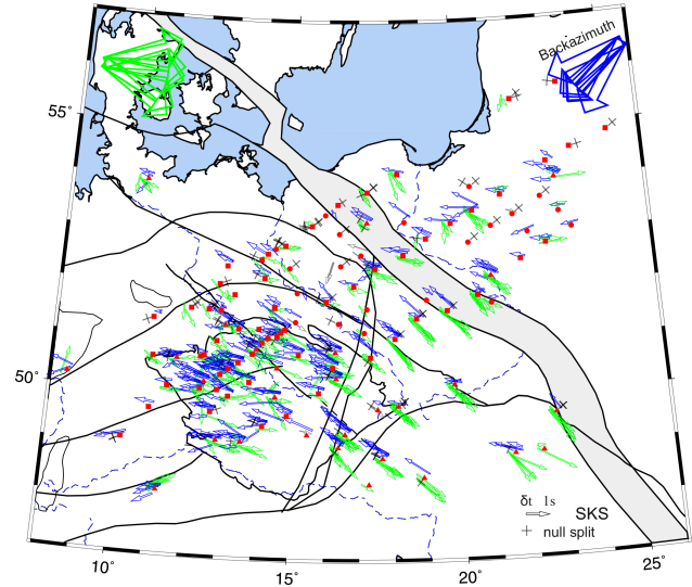
Figure 7. Fast shear-wave polarizations ( \psi , \delta t ) evaluated in the LQT coordinate system presented at ray-piercing points at depth of 80 km. The arrows mark azimuths \varphi of the polarized fast split shear waves and point in down-dip directions. See also Fig. 3 and related text.
