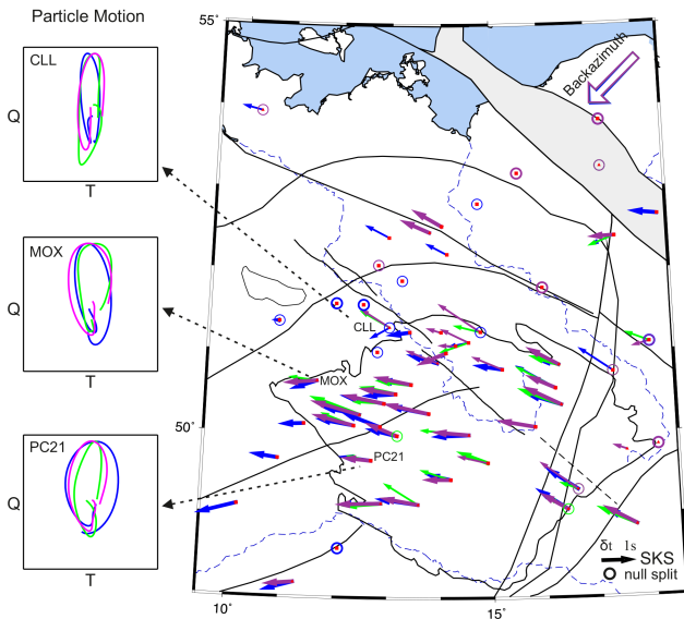
Figure 12. Shear-wave polarizations evaluated at a part of the PASSEQ array from recordings of three events. Splitting parameters evaluated from narrow PM of waves arriving from very close directions differ at station CLL, while we get identical splitting parameters from the broad PM at e.g. station PC21. Complex structures can affect significantly the splitting parameters of waves arriving even from very close directions.
