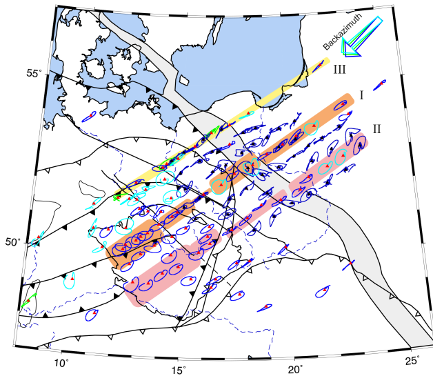
Figure 9. PMs for three events from the NE (the same as in Fig. 8). To emphasize variations of the PM across and along the TESZ, three profiles of the BB stations are marked by coloured bands, whose widths are in relation to the width of the PM ellipses: orange – three areas of broad PMs (in the BM, TESZ/TTZ and EEC) along profile I; red – broad PMs in the BM, followed by narrow PMs, getting gradually broader in the EEC along profile II; yellow – mostly linear PMs along profile III.
