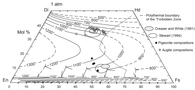
Fig. 3. Graphical pyroxene geothermometer after Lindsley (1983). Pigeonite and augite data from Creaser and White (1991), Stewart (1994) and this study indicate magmatic temperatures between 900 °C and 1110 °C for the upper Gawler Range Volcanics.
