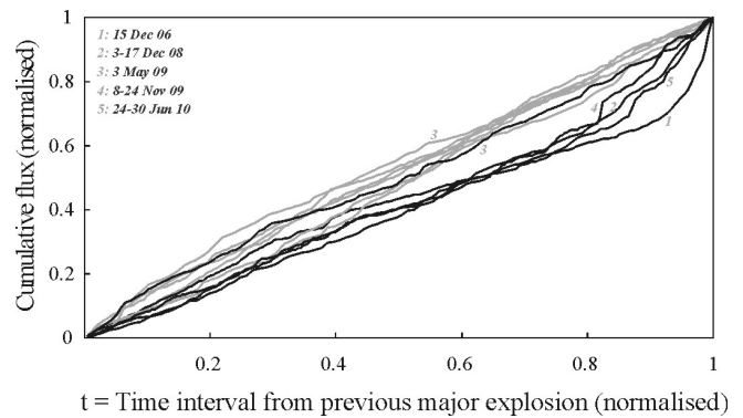
Fig. 5. Normalised cumulative CO 2 (black curve) and SO 2 (grey curve) flux trends for 5 periods of activity of Stromboli. The periods over which the cumulative curves were drawn were all selected in order to start ( t = 0 ) on the day after the previous explosive event and to end ( t = 1 ) with one (or more) major explosions (numbers 1–5 denote the specific explosion(s) occurring at t = 1 ). Curves 5 for CO 2 and SO 2 are totally analogous, in the normalised form, to those shown in Fig. 4a, and have t = 0 on 13 March and t = 1 on 30 June. The time interval between 0 and 1 is thus the period over which a complete cycle of gas segregation-gas leakage can occur. The 5 sets of normalised cumulative curves show similar shapes which indicate a reproducible degassing regime prior to each major explosion and, hence, a common recurrent source mechanisms for these events. A less pronounced difference between SO 2 and CO 2 cumulative trends is observed for case 3, implying that while the involved source processes were probably the same, a smaller volume of CO 2 was accumulating/leaking prior to the 3 May 2009 event.
