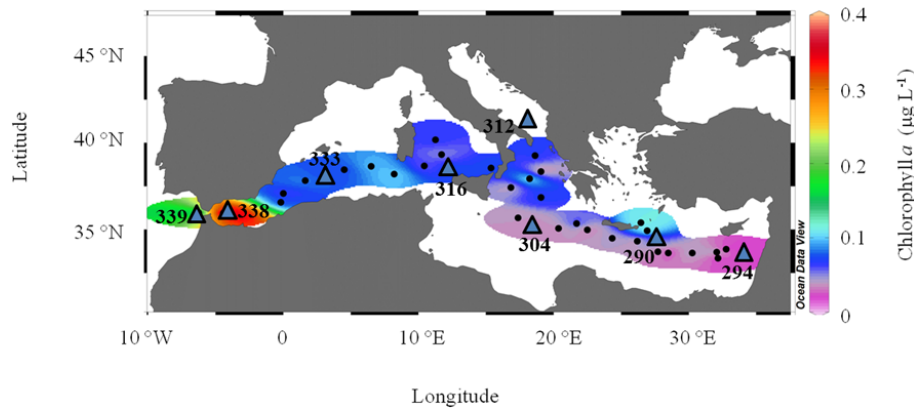
Fig. 1. Map of the sampling locations (triangles): NW Levantine basin (St. 290), anticyclonic Shikmona eddy (St. 294), Ionian Sea (St. 304), Adriatic Sea (St. 312), Tyrrhenian Sea (St. 316), Alboran Sea (St. 333), Strait of Gibraltar (St. 338) and Gulf of Cadiz (St. 339). Background (circle): spatial distribution of chlorophyll a concentrations in surface waters (6–8 m) along the R/V Meteor M84/3 cruise track ( n = 94 ).
