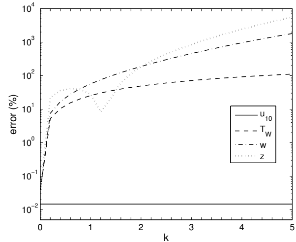
Fig. 13. Optimal k for wind speed ( u_{10} ), water temperature ( T_w ), current velocity ( w ) and depth ( z ). All n_i = 5 and \Theta_i = 5 . The \delta_4 = 2\ km\ h^{-1} ( u_{10} ), \delta_8 = 1.8\ ^\circ C ( T_w ), \delta_{10} = 0.7488\ hm\ h^{-1} ( w ) and \delta_{11} = 1.29\ dam ( z ).
