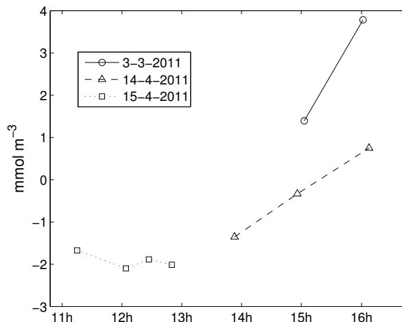
Fig. 11. \Delta CO 2 for the three sampled time series.
