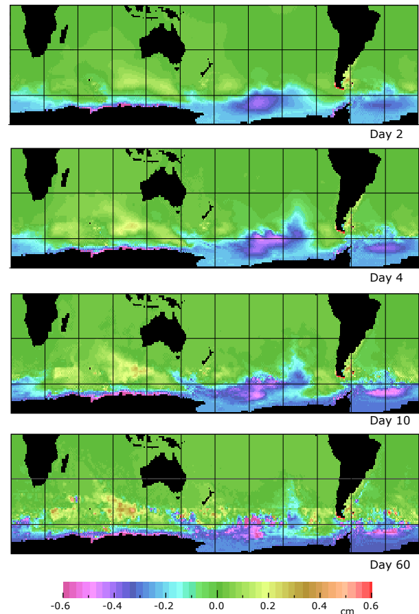
Fig. 5. Difference in sea level between the perturbation run and the control run after two days, four days, ten days and sixty days. Grid lines at 30^\circ degree intervals.
