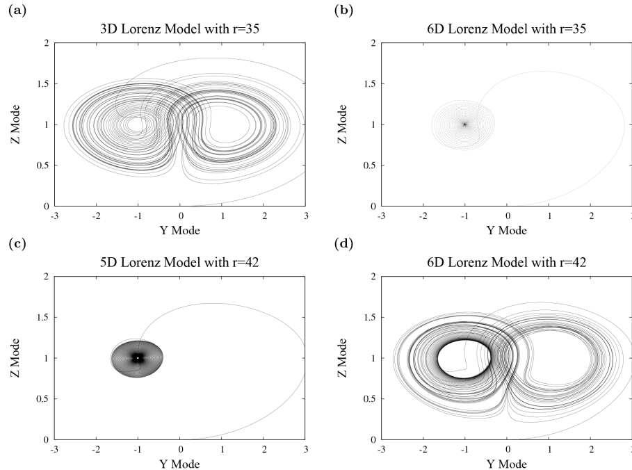
Figure 2. (Y, Z) plots in the 3DLM (a) and 6DLM (b) with r = 35 ; and 5DLM (c) and 6DLM (d) with r = 42 . Lorenz strange attractors appear in (a) and (d). All of the solutions are normalized by the the corresponding critical points, namely, Eq. (21) of Shen14 for the 3DLM and Eq. (19) of Shen14 for the 5DLM and 6DLM.
