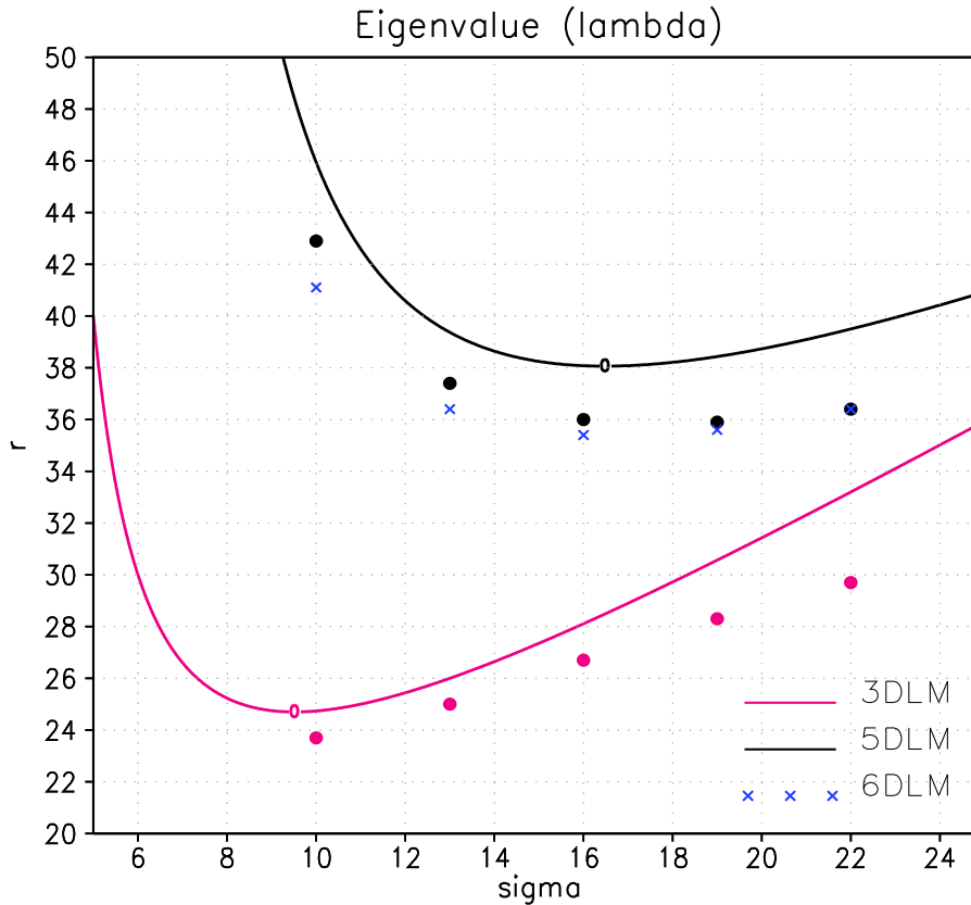
Figure 7. The r_c of the 6DLM as a function of \sigma . The r_c , shown by blue multiplication signs ( \times ) are determined by the eLEs of the nonlinear 6DLM. The pink and black lines indicate a constant contour of Re(\lambda) = 0 for the linear 3DLM and 5DLM, respectively, indicating the corresponding r_c , based on a linear stability analysis. Solid circles with the same color scheme indicate a r_c , determined by the eLEs analysis with \Delta r = 0.1 in the corresponding nonlinear LM.
