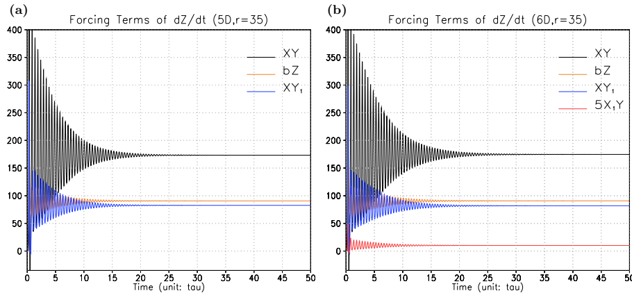
Figure 3. Forcing terms of dZ/d\tau with r = 35 , which are from Eq. (12) for the 5DLM of Shen (2014) (a) and Eq. (10) for the 6DLM (b) , respectively. The black and orange lines represent XY and bZ , respectively, while the blue and red lines represent XY_1 and 5X_1Y , respectively.
