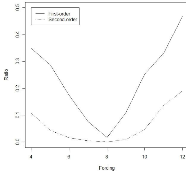
Fig. 2. The proportions of residual ratios of the first-order and second-order Taylor expansions over the nonlinear observation operator \mathbf{x}_{i,k}^t \exp\{0.1\mathbf{x}_{i,k}^t\} that fall outside the interval [-0.1, 0.1] , as a function of forcing F .
