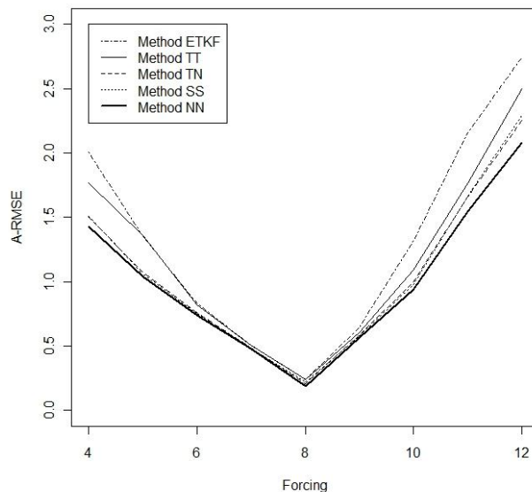
Fig. 1. Time-mean values of the A-RMSE as a function of forcing F for different assimilation methods on Lorenz-96 model. ETKF: traditional ETKF described in the last paragraph of Sect. 2.1; TT: tangent-linear approximation in both inflation (Eq. 17) and optimization (Eq. 20) (thin solid line); TN: tangent-linear approximation in inflation (Eq. 17) and nonlinearity in optimization (Eq. 10) (dashed line); SS: second-order Taylor approximation in both inflation (Eq. 24) and optimization (Eq. 27) (dotted line); NN: nonlinearity in both inflation (Eq. 5) and optimization (Eq. 10) (thick solid line). The ensemble size is 30.
