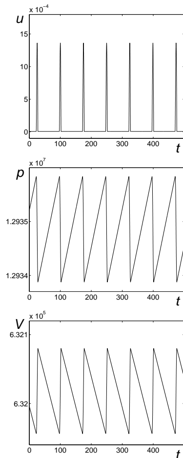
Figure 3. Time series of the cycle shown in Fig. 2: u (m s -1 ), p (Pa) and V (m 3 ) as functions of time t (s).
