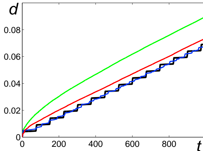
Figure 7. Displacement d (m) as a function of time t (s) under the influence of F -noise: deterministic case (black), \varepsilon = 10^{-4} (blue), \varepsilon = 5 \times 10^{-4} (red), and \varepsilon = 10^{-3} (green).
