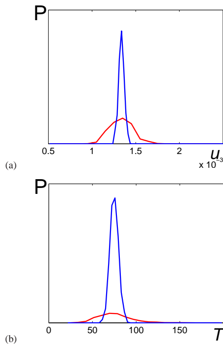
Figure 9. Influence of Q -noise for \delta = 0.5 (blue), and \delta = 2 (red): (a) probability density functions of u coordinates ( \text{m s}^{-1} ), (b) probability density functions of the period T (s).
