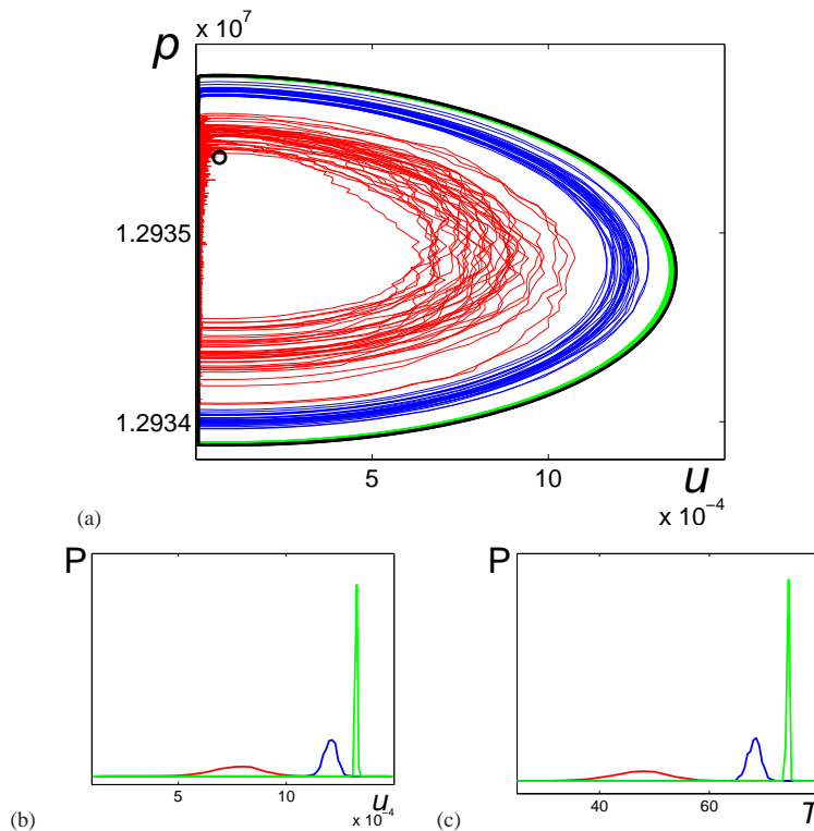
Figure 5. Stochastic cycles for \varepsilon = 10^{-6} (green), \varepsilon = 10^{-5} (blue), and \varepsilon = 5 \times 10^{-5} (red): (a) random trajectories p (Pa) vs. u ( \text{m s}^{-1} ), (b) probability density functions of u coordinates ( \text{m s}^{-1} ), (c) probability density functions of the period T (s).
