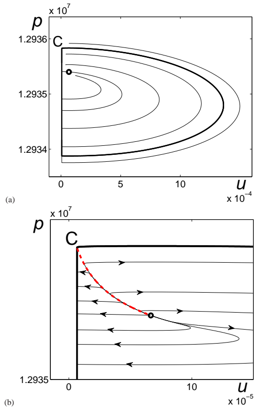
Figure 2. (a) Projection of the phase portrait of the deterministic system, p (Pa) vs. u ( \text{ms}^{-1} ). (b) illustrates an enlargement near unstable equilibrium (open circle). The dashed red line is a pseudo-separatrix. Physical parameters of the system under consideration are (Iverson et al., 2006): B = Q = 2 \text{ m}^3 \text{ s}^{-1} , m_0 = 3.6 \times 10^{10} \text{ kg} , A = 30\,000 \text{ m}^2 , p_0 = 12\,936 \times 10^3 \text{ Pa} , \alpha_1 = 10^{-7} \text{ Pa}^{-1} , \alpha_2 = 10^{-9} \text{ Pa}^{-1} , F_0 = 3528 \times 10^7 \text{ kg ms}^{-2} , u_{\text{ref}} = 0.1Q/A = 66\,667 \times 10^2 \text{ ms}^{-1} , V_0 = 6.32 \times 10^5 \text{ m}^3 , c = 1.7 \times 10^{-4} , g = 9.8 \text{ ms}^{-2} , \rho_0 = \rho_r = 2000 \text{ kg m}^{-3} , \kappa = 0 .
