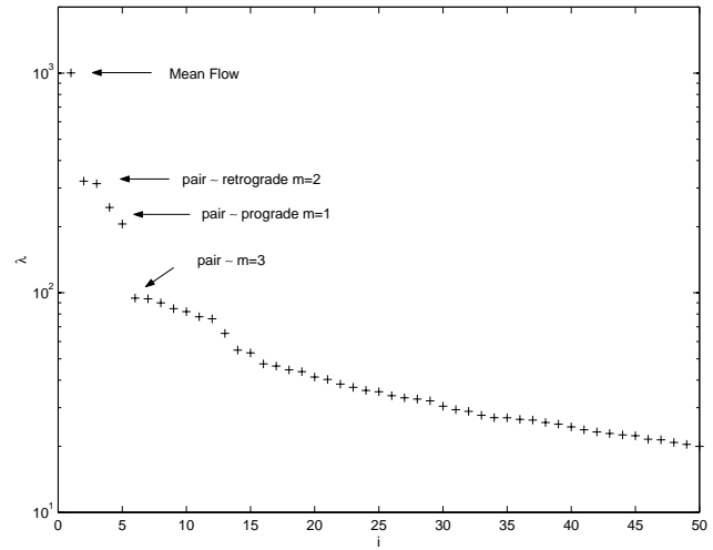
Fig. 6. Singular values for the EOF analysis of the set of full field data.
