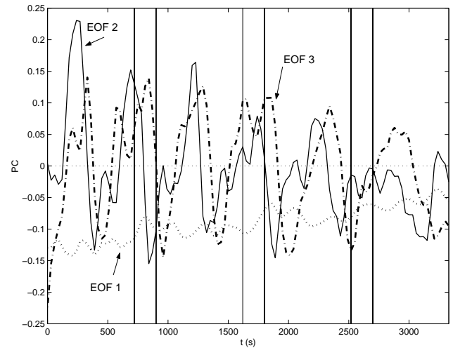
Fig. 14. Principal Components from the EOF analysis of the set of rotated eddy fields. All PCs are scaled by their singular values.
