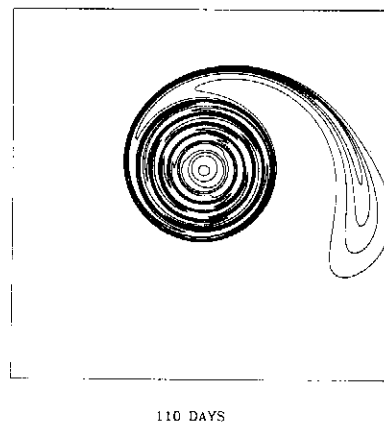
Fig. 2. The final ( t = 110 \text{ days} ) snapshot of eddy (4): tracer concentration.
