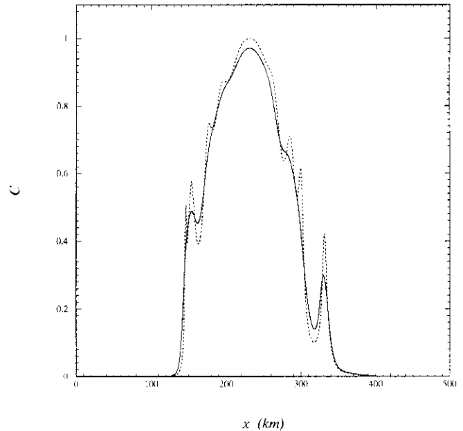
Fig. 13. The cross-section of the concentration field for eddy (18) after 35 days. The solid/dotted lines show the profiles computed using the diffusive/non-diffusive models, respectively.
