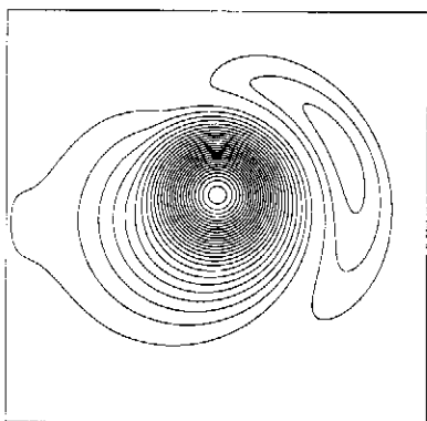
Fig. 6. The final ( t = 110 days) snapshot of eddy (4): the streamfunction.
