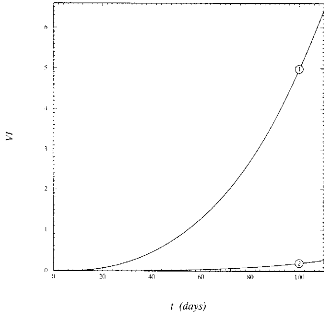
Fig. 8. The “variability indicator” vs. time for eddy (4). (1) tracer concentration; (2) potential vorticity.
