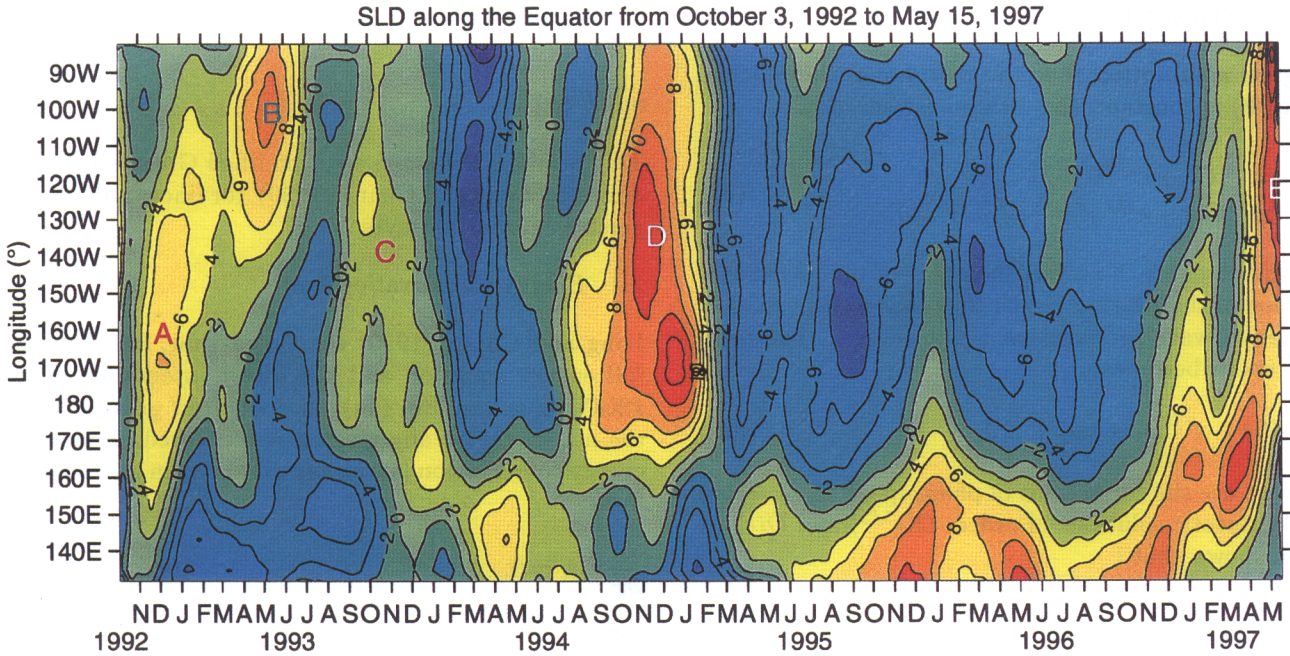
Fig. 1. Longitude-time contour plot of low-pass-filtered TOPEX/POSEIDON sea level deviation (SLD). The interval between two adjacent contours is 1 cm. The major positive peaks are coded by capital letters.
