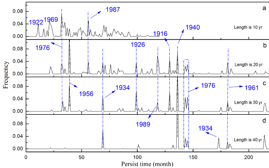
Figure 9. Distribution of the abrupt change persist time with the start moment. (a–d) show the different conditions in which the length of the sub-sequence are set, which are 10a, 20a, 30a, and 40a. The x axis refers to the persist time of the abrupt change, the y axis refers to the frequency of the abrupt changes that satisfies the conditions, and the characters mark the start moments of each abrupt change process.
