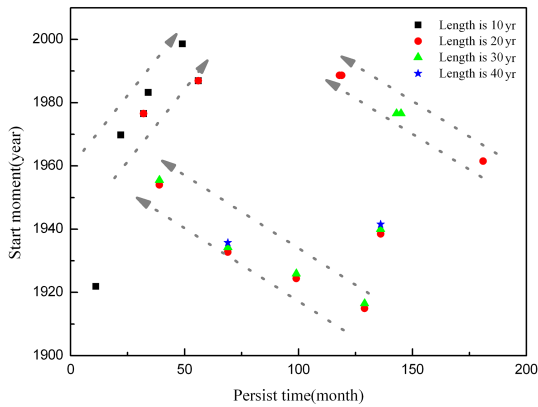
Figure 10. Abrupt changes start at different moments than their persist times. The x axis refers to the persist time of each abrupt change process, and the y axis refers to the start moment.
