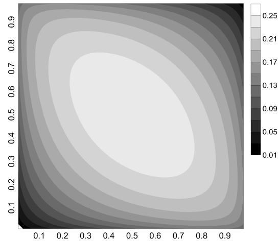
Figure 4. The relationship parameter \chi and parameters \alpha, \beta , where the x axis is parameter \alpha , the y axis is parameter \beta and the contour is parameter \chi .
