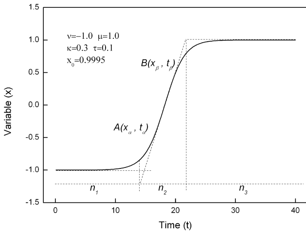
Figure 3. The abrupt change process and its sections. The three sections are as follows: period before the abrupt change, period of abrupt change process, and period after abrupt change.
