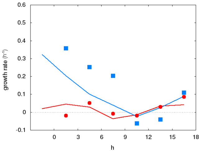
Figure 3. Growth rates of forecast errors for the two control trajectories of Fig. 1 and the corresponding leading bred vector. Times indicated on the x axis correspond to UTC times on 26 September 2006. Breeding parameters: period 30 min, amplitude 0.36 (red dots) for trajectory 18H (large initial error, red line); period 15 min, amplitude 0.100 (blue squares) for trajectory R21 (small initial error, blue line).
