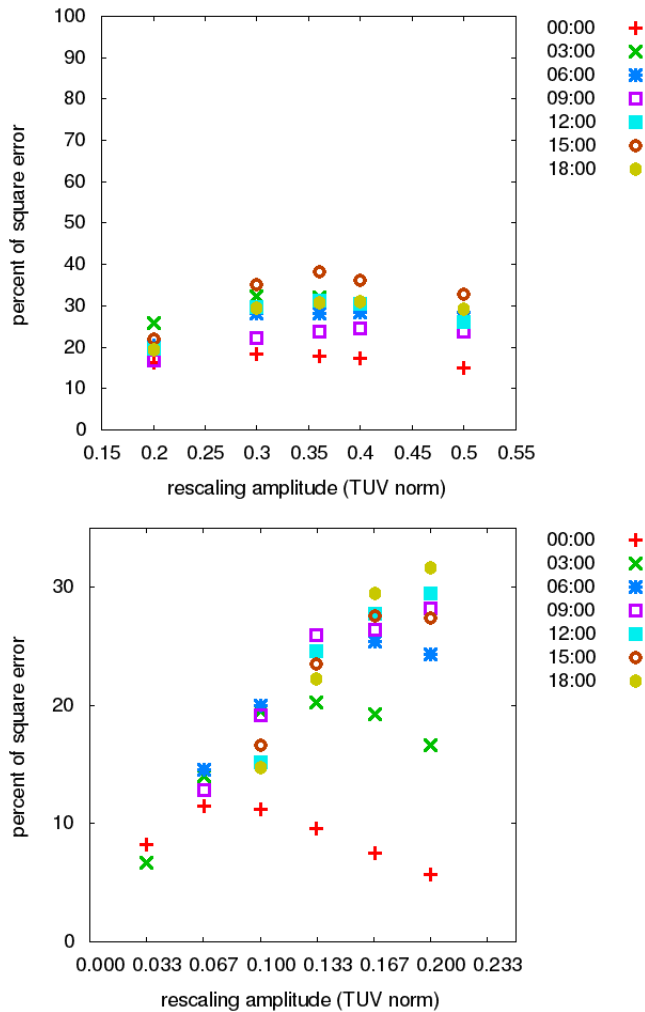
Figure 5. Square norm of error orthogonal projection onto the subspace of the first 12 bred vectors (percentage of error square norm), as in Fig. 4, but plotted here as a function of rescaling amplitude. Different symbols are used in each panel to mark different times (UTC, 26 September 2006). Top panel: control trajectory 18H (large initial error), longer rescaling period 30 min. Bottom panel: control trajectory R21 (small initial error), shorter rescaling period 15 min. The same data are plotted as a function of lead time in Fig. 4.
