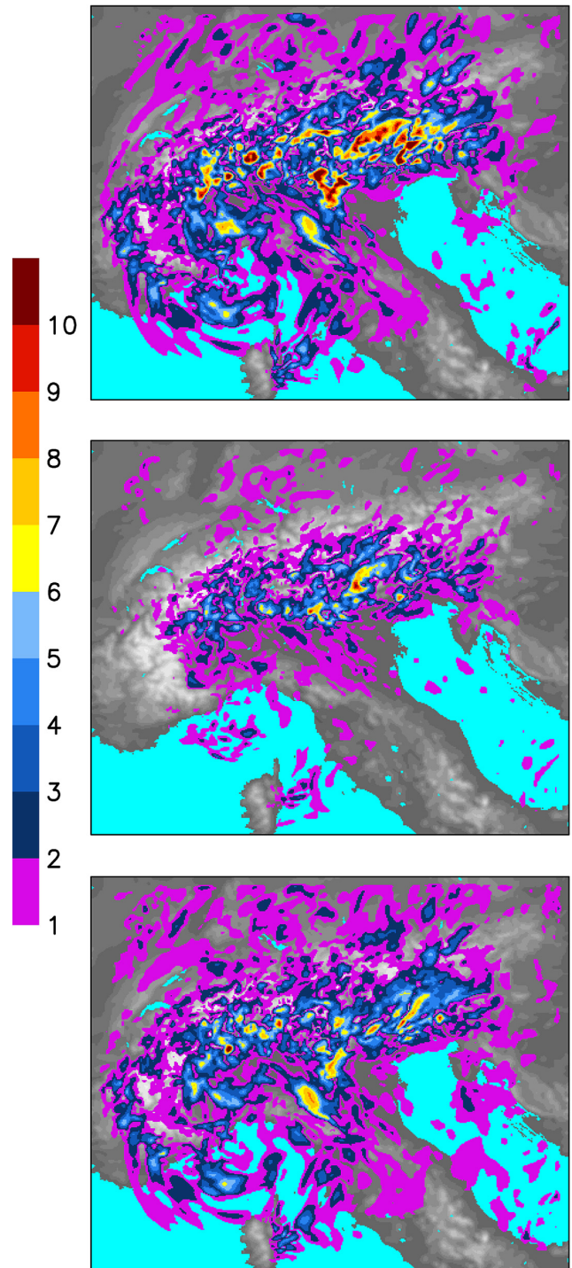
Figure 7. Maps of error at 03:00 UTC on horizontal velocity (norm of two-dimensional vector differences, \text{ms}^{-1} ). Top: error of control state 18H (trajectory started with large initial error). Middle: projection of the error onto the 12 BV subspace. Bottom: difference between the two above fields, i.e. error of the restart state of Fig. 8.
