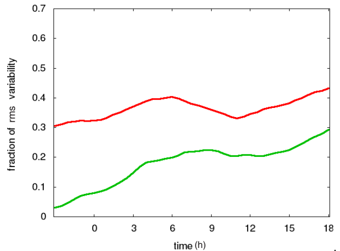
Figure 1. The rms forecast error of control trajectories with different initial errors. Times indicated on the x axis correspond to UTC times of 26 September 2006. Values on the y axis are non-dimensional (TUV norm defined in the text) and are expressed as fractions of natural variability. Red: trajectory labelled 18H (actually starting at 18:00 UTC on 25 September), which at 21:00 UTC has error 0.3, of the order of the present-day analysis error. Green: trajectory labelled R21, obtained from the previous one by rescaling, at 21:00 UTC on 25 September, its error to 0.03, i.e. 1 order of magnitude smaller than the present-day analysis error
