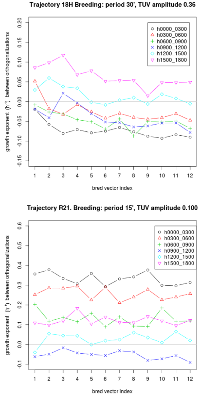
Figure 2. Growth rates of the 12 bred vectors at different forecast times, as a function of the bred vector index (the growth rate has been averaged over 3 h intervals, as indicated in the legend box). Different colours refer to different forecast times. As indicated in the panel titles, the BVs are constructed differently for trajectory 18H (large initial error, top panel) and for trajectory R21 (small initial error, bottom panel).
