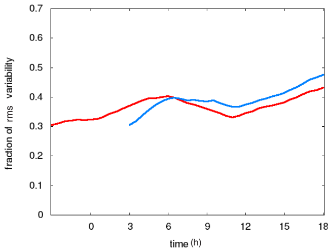
Figure 8. Red: rms error evolution of the 18H control trajectory, same as in Fig. 1. Blue: error of the trajectory restarted after subtraction of the orthogonal error component on the 12 bred vectors' subspace. Times indicated on the x axis correspond to UTC times on 26 September 2006.
