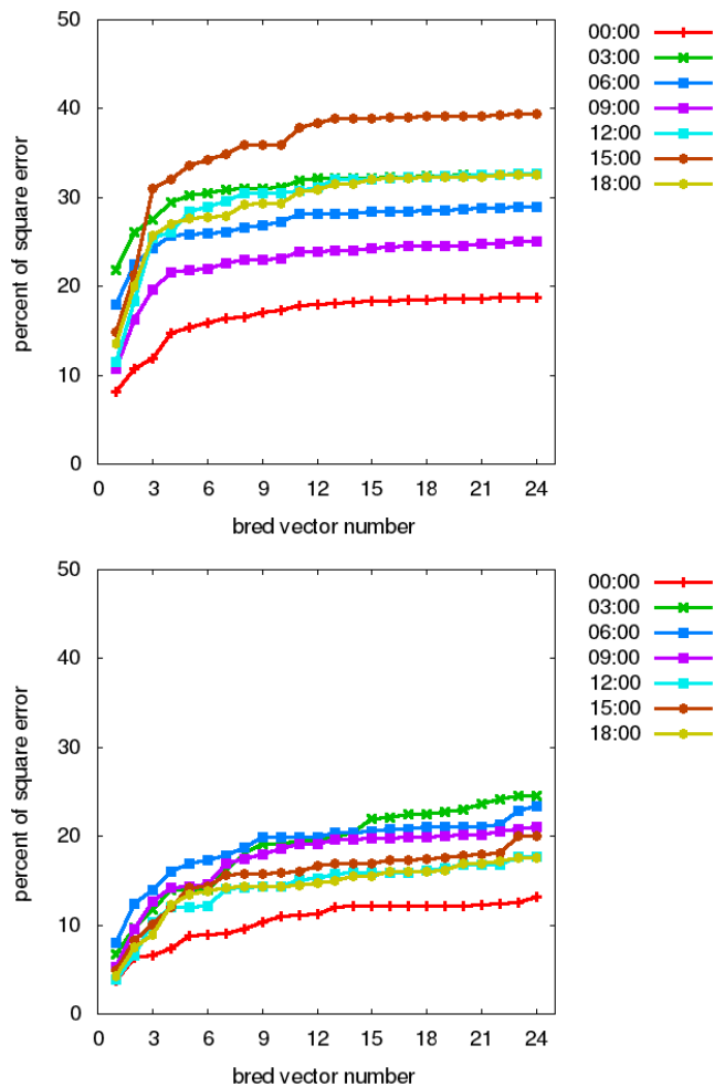
Figure 6. Square norm of error orthogonal projection onto subsets of bred vectors (percentage of error square norm) as a function of subspace dimension. Different curves in each panel correspond to different times (UTC, 26 September 2006). Top panel: control trajectory 18H (large initial error), rescaling period 30 min, rescaling rms TUV norm 0.36. Bottom panel: control trajectory R21 (small initial error), rescaling period 15 min, rescaling rms TUV norm 0.10.
