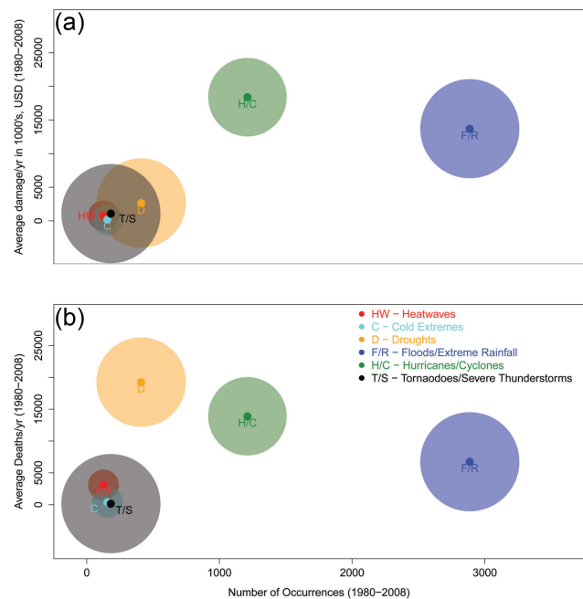
Figure 1. Frequency and severity of hydrometeorological hazards, indicated as damages in US dollars (a) and annual fatalities (b), along with their uncertainties in our current understanding in a climate change context. Damage and fatality data are taken from the UN Office for Disaster Risk Reduction (UNISDR) at PreventionWeb ( http://www.preventionweb.net/english/hazards/ ) averaged over 1980–2008. The uncertainties are represented by the size of the bubbles with larger circles indicative of greater uncertainty and are derived from the IPCC confidence and likelihood estimates (Field et al., 2012).
