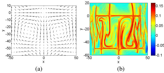
Fig. 1. (a) Vector field and (b) FTLE field of the model given by Eq. (2) for two gyres with A = 10 , \mu = 0.005 , \varepsilon = 0.1 , \psi = 0 , I = 0.01 , and s = 50 . LCS are characterized by regions with maximum FTLE measures (denoted by red). In 2-D flows, regions with maximum FTLE measures correspond to 1-D curves.
