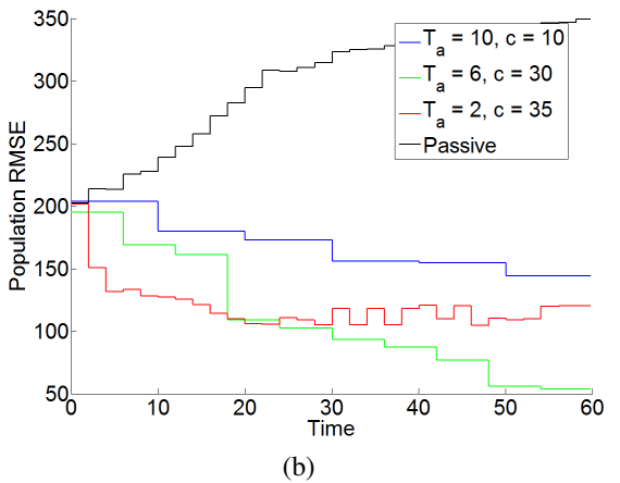
Fig. 14. (a) Final RMSE for different values of c and T_a using the experimental flow field. T_c/T_a = 0.8 is kept constant throughout. (b) RMSE over time for select c and T_a parameters on an experimental flow field. The duty cycle T_c/T_a = 0.8 is kept constant throughout.
