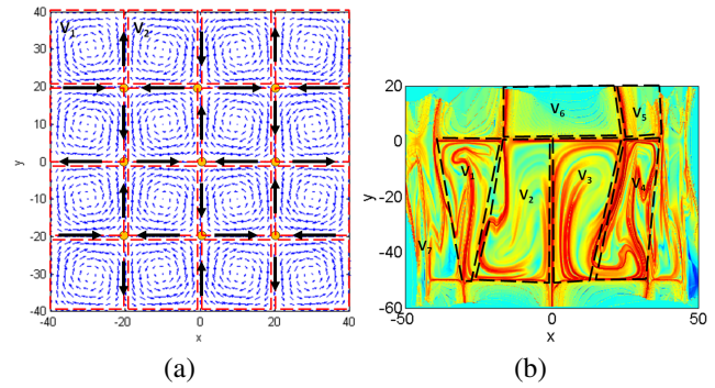
Fig. 2. Two examples of LCS-based cell decomposition of the region of interest assuming a flow field given by Eq. (2). These cell decompositions were performed manually. (a) A 4 \times 4 time-independent grid of gyres with A = 0.5 , \mu = 0.005 , \varepsilon = 0 , \psi = 0 , I = 35 , and s = 20 . The stable and unstable manifolds of each saddle point in the system is shown by the black arrows. (b) An FTLE based cell decomposition for a time-dependent double-gyre system with the same parameters as Fig. 2.
