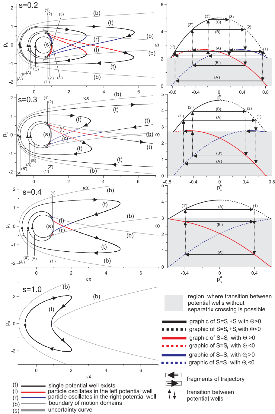
Fig. 5. Particle trajectories in the phase plane of the slow variables are shown for four values of the parameter s (the left column). Corresponding profiles of S_{l,r} and S are shown in the right column.
