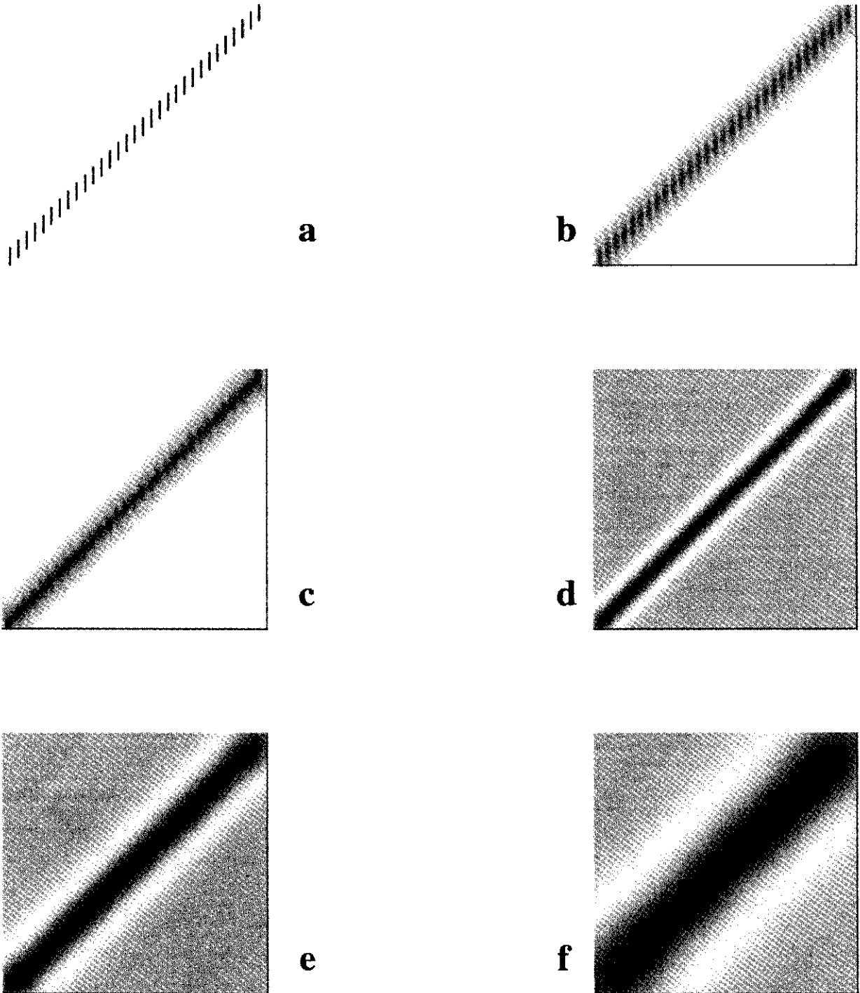
Fig. 5: Isotropic wavelet analysis of Fig. 4 (reproduced in 5a). Scales of analysis are respectively a = 2 ( b ), 4( c ), 8( d ), 16( e ) and 32( f ) pixels. Wavelet coefficients have been rescaled between 0 (white) and 1 (darkest grey).
