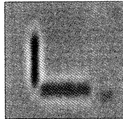
Fig. 7b: Anisotropic wavelet analysis of Fig. 6, with \alpha = 4 and \sigma = 2 . The azimuth of the wavelet is \pi/2 such that the long axis is vertical. Wavelet coefficients are rescaled to fit the interval between 0 (white) and 1 (darkest grey).
