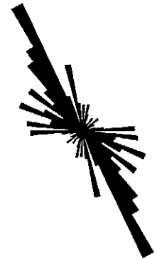
Fig. 15: OAWC method applied to Map V. The original picture is shown in case a. Wavelet coefficients are rescaled between 0 (white) and 1 (darkest grey). Black dots represent the VRL's. Rose diagrams on the right are associated either with the original pattern or the VRL's (from b to f). Scales of analysis are respectively 2(b), 4(c), 8(d), 16(e) and 32 (f) pixels.
