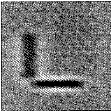
Fig. 7a: Anisotropic wavelet analysis of Fig. 6, with \alpha = 4 and \sigma = 2 . The azimuth of the wavelet is 0 such that the long axis is horizontal. Wavelet coefficients are rescaled to fit the interval between 0 (white) and 1 (darkest grey).
