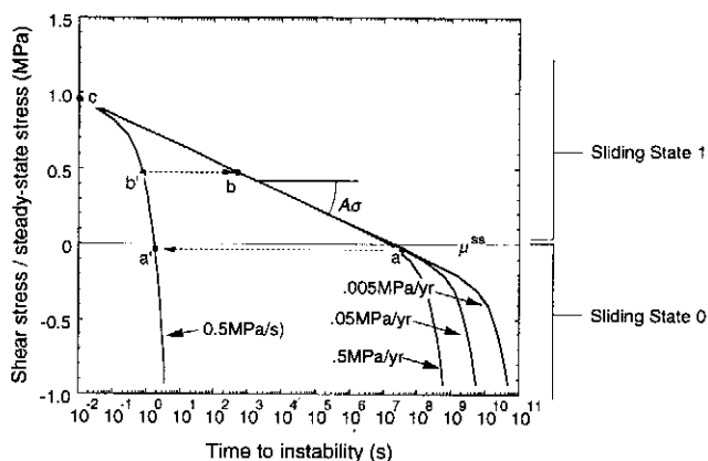
Fig. 2. Effect of initial stress and stressing rate on the time to instability for state 1 slip from Eq.(14). The curve \dot{\tau} = 0.5\text{MPa/s} illustrates conditions near a earthquake source during earthquake slip. A loading rate \dot{\tau} = 0.05\text{MPa/year} is equivalent to tectonic deformation of 1\text{cm/year} . The effect of an earthquake loading step on time to instability is illustrated by a fault segment which is initially about 1 year from instability at \dot{\tau} = 0.05\text{MPa/year} (point a). A one second stress application at \dot{\tau} = 0.5\text{MPa/s} followed by a return to \dot{\tau} = 0.05\text{MPa/year} reduces the time instability to about 4 minutes (from a' to b to b'). A two second application of stress at \dot{\tau} = 0.5\text{MPa/s} reduces the time to 0.01s (point c) which corresponds to failure during the earthquake. Model conditions are \sigma = 15\text{MPa} , D_c = 0.0001\text{m} , A = 0.003 , B = 0.015 and \theta = 10^8\text{s} .
