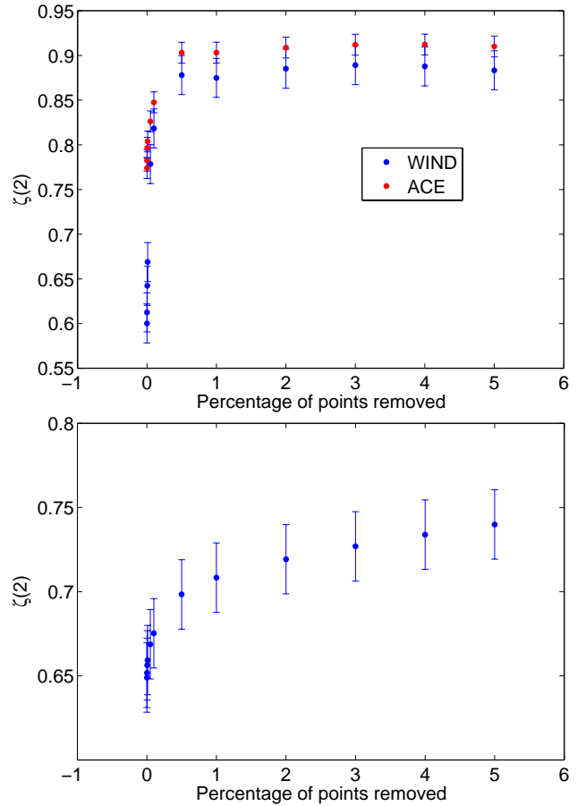
Fig. 7. Exponent of the second moment \zeta(2) vs. the percentage of points excluded for (a) WIND and ACE at solar maximum and (b) WIND at solar minimum (after Kiyani et al., 2007).
