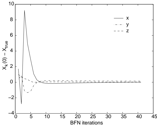
Fig. 1. Difference between the k th iterate X_k(0) and the exact initial condition X_{true} for the 3 variables versus the number of BFN iterations.
