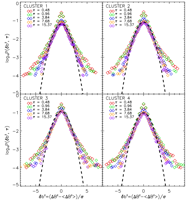
Fig. 9. PDFs of fluctuations of the magnetic energy measured by the four Cluster satellites in the magnetosheath. PDFs have been scaled with respect to their \sigma(\tau) .
