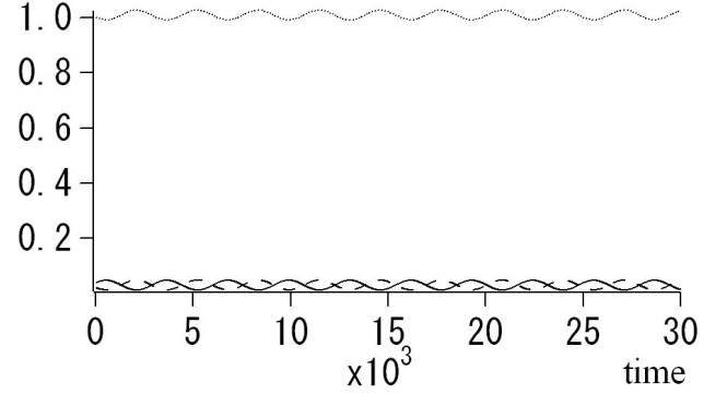
Fig. A2. Same as Fig. A1 except that the initial condition here is N_2 \gg N_1, N_3 . The broken, dotted, and solid lines indicate N_1, N_2 , and N_3 , respectively. The system is “stable” in the sense that variations of N_1, N_2 , and N_3 are small.
