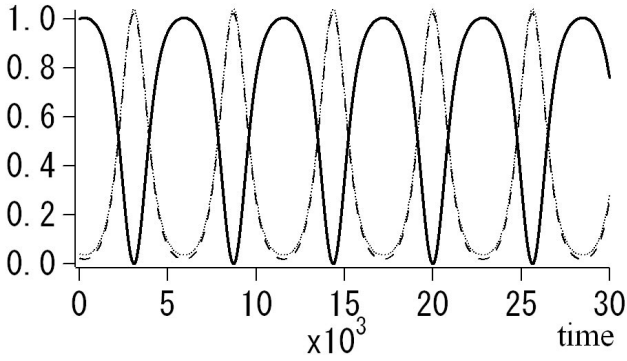
Fig. A1. Time evolution of N_j with the initial condition, N_3 \gg N_1, N_2 . The broken, dotted, and solid lines indicate N_1, N_2 , and N_3 , respectively. The system is “unstable” in that the “quanta” originally stored in mode 3 are re-distributed to modes 1 and 2 within an instability time scale ( \sim 3000 ).
