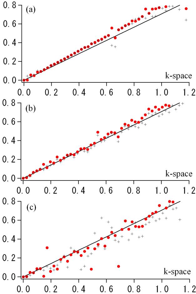
Fig. 16. Numerically computed frequency \dot{\phi}_k^u (red circles) and \dot{\phi}_k^\rho (black crosses) versus the wave number k at (a) t=350 , (b) t=500 , (c) t=720 . When 0 < t \lesssim 500 , the longitudinal modes \dot{\phi}_k^u , \dot{\phi}_k^\rho are distributed around a line slightly (but distinctly) above the sound wave branch (solid black line). The former may be called the “ponderomotive density fluctuation” branch. As later times, however, we find that the longitudinal wave frequencies are re-distributed around the sound branch.
