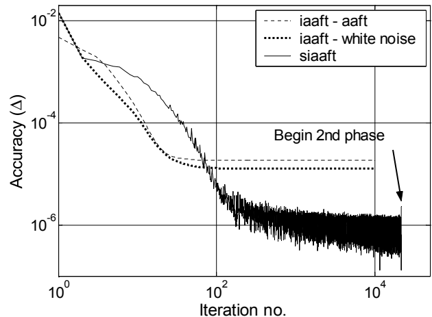
Fig. 3. The convergence of the algorithms as a function of the number of iterations. As test statistics we used a fractal time series ( N=8192 ) with a power law power spectrum with an exponent of -5/3 and an exponential amplitude distribution. The three line types represent the IAAFT algorithm starting with white noise (thick dashes), the IAAFT algorithm starting with an AAFT surrogate (thin dashes) and the SIAAFT algorithm (noisy full line).
