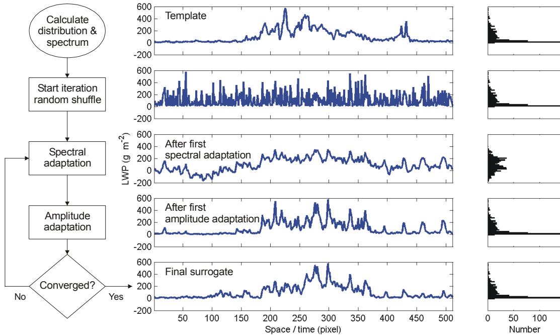
Fig. 2. The Iterative Amplitude Adjusted Fourier Transform algorithm illustrated with a LWP measurement. The left column is the flow diagram of the algorithm, the middle column shows example LWP time series, and the right column are the histograms of the LWP time series. For the explanation of the algorithm, see Sect. 2. Figure reprinted with permission from: Venema et al. (2006).
