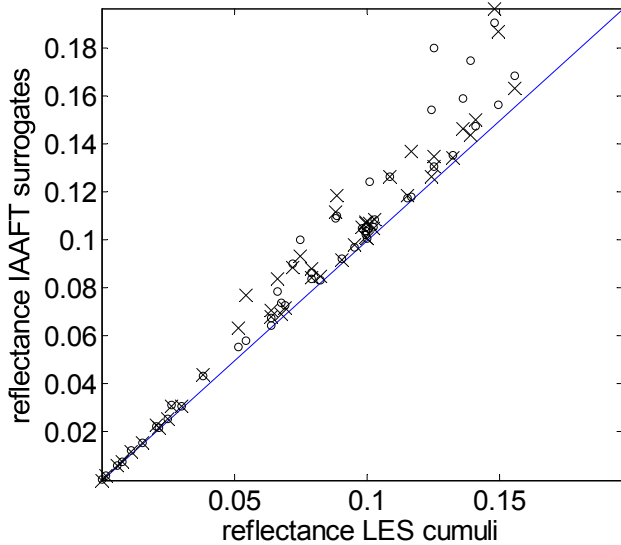
Fig. 1. The reflectance of sparse cumulus clouds compared with the reflectance ( R ) of their IAAFT surrogates. The surrogate cumulus clouds have a bias toward a too high reflectance. The accuracy was improved by repeating the calculation and selecting the best converged surrogate. For every cumulus cloud, we have generated two surrogate clouds. The most accurate cloud (average \Delta=3.4\times 10^{-3} ; see Eq. 4) is denoted by a cross, the least accurate (average \Delta=4.7\times 10^{-3} ) one by a circle. Even in this optimised set of clouds, the accurate surrogates have a little less bias ( \Delta R=8.1 \cdot 10^{-3} ), than the less accurate ones ( \Delta R=8.9\times 10^{-3} ).
