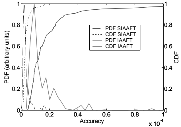
Fig. 6. The Probability Density Functions (PDF) and the Cumulative Distribution Functions (CDF) of the accuracy ( \Delta ) of the IAAFT and the SIAAFT algorithm. The SIAAFT algorithm used an iteration threshold of 1000 and the test function described in Fig. 3. An ensemble of one hundred surrogates was generated to calculate these statistics. Three outliers of the IAAFT algorithm, were not plotted, to get a clearer plot.
