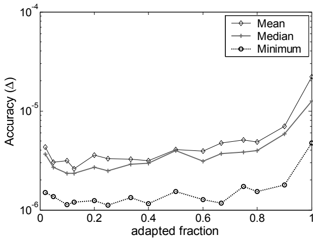
Fig. 5. The accuracy of the SIAAFT algorithm as a function of the fraction of values that is adjusted in the amplitude adjustment. This was calculated with the test function described in Fig. 3. The SIAAFT algorithm with an adjusted fraction of one is similar to the IAAFT algorithm. The SIAAFT algorithm used an iteration threshold of 10^3 . An ensemble of one hundred surrogates was utilised to calculate the statistics.
