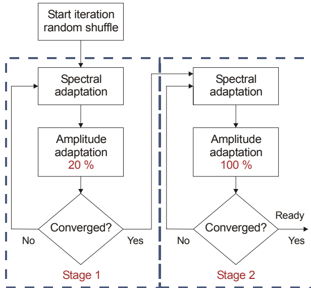
Fig. 4. The flow diagram of the Stochastic Iterative Amplitude Adjusted Fourier Transform algorithm. The two stages are similar to the original IAAFT algorithm and differ in their treatment of the amplitude adjustment.
