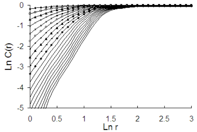
Fig. 11. Ln C(r) vs. Ln r plot for the series, after removing noise, observed at the Arkansas river. The curves are shown in ascending order of embedding dimension, m=1, 2, \dots, 20 from top to bottom.
