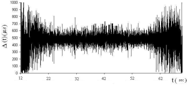
Fig. 3. Time series of time intervals between consecutive maximum amplitudes of acoustic signals (waiting times) in consecutive \pi -periods of external forcing.
