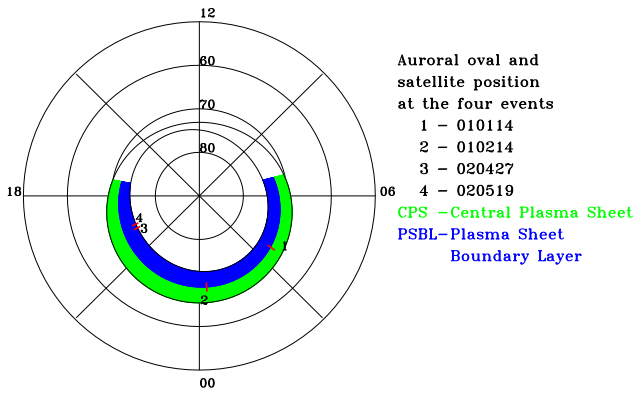
Fig. 3. Overview of the locations of the four electric field events, with respect to the auroral oval and plasma boundaries. The corresponding Cluster orbit segments have been projected to the northern auroral ionosphere using an Invariant Latitude-Magnetic Local Time polar diagram. Events 1 and 2 were encountered at the boundary between the plasma sheet boundary layer (blue color) and the central plasma sheet (green color) and events 3 and 4 were encountered at the polar cap boundary.
