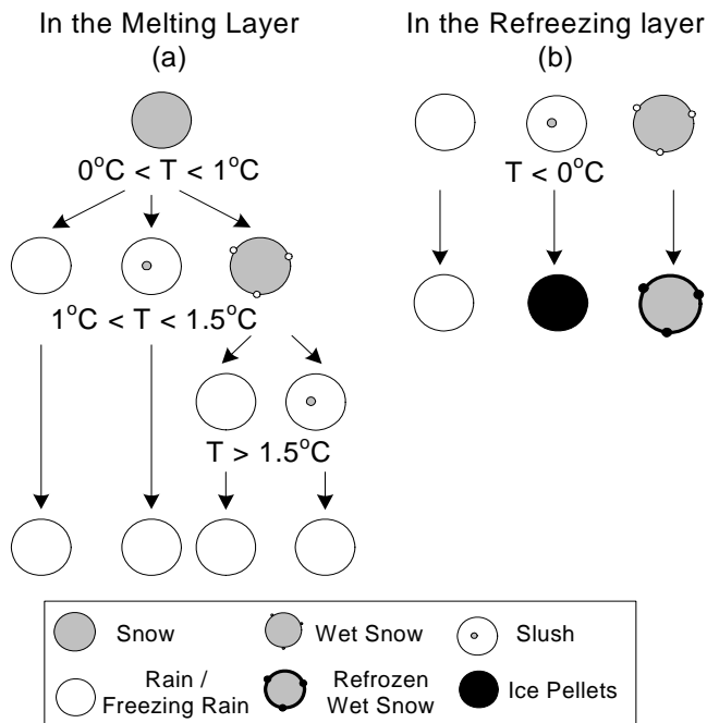
Fig. 2. A schematic of the different types of precipitation formed under various temperatures. (a) The melting of snowflakes into slush, wet snow and rain within the melting layer. Wet snow melts into rain and slush and eventually slush melts into rain. (b) The refreezing of liquid and partially liquid particles. The rain changes into freezing rain, slush into ice pellets and wet snow into refrozen wet snow within the subfreezing layer below the melting layer.
