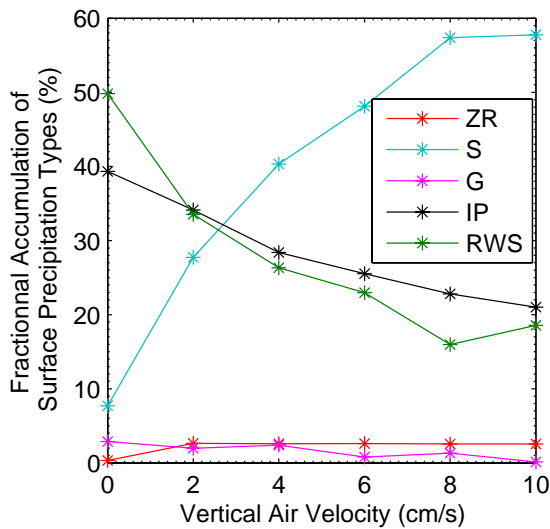
Fig. 9. The fractional accumulation (%) of precipitation types at the surface through 240 min for various values of vertical air velocities ( w_{max} ). The symbols for the precipitation types are freezing rain (ZR), snow (S), graupel (G), ice pellets (IP) and refrozen wet snow (RWS).
