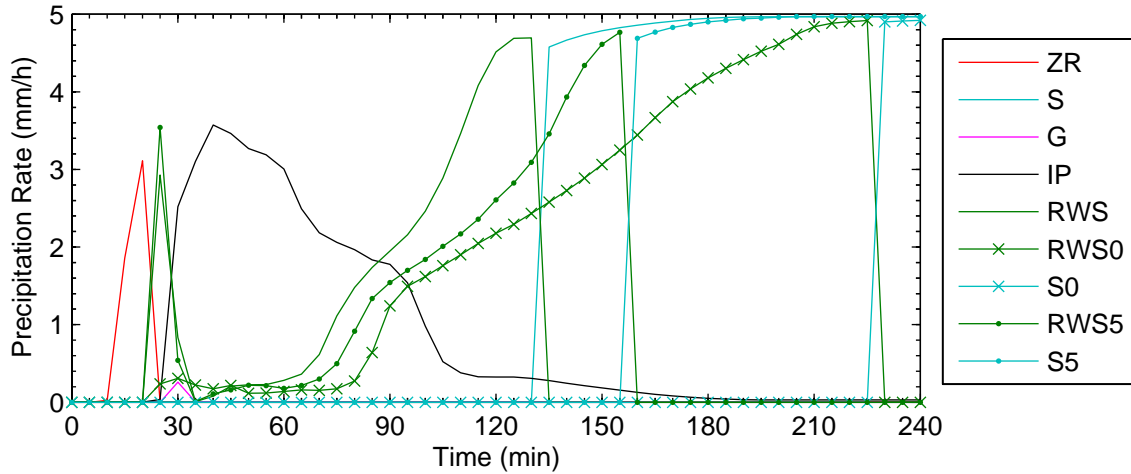
Fig. 8. The evolution of all the precipitation types are for w_{max}=10 cm/s and the evolution of snow for w_{max}=0 cm/s and w_{max}=5 cm/s. The symbols for the precipitation types are freezing rain (ZR), snow (S), graupel (G), ice pellets (IP), refrozen wet snow (RWS), refrozen wet snow (RWS5) and snow (S5) when w_{max}=5 cm/s (Eq. 11), refrozen wet snow (RWS0) and snow (S) when w_{max}=0 cm/s (Eq. 11).
