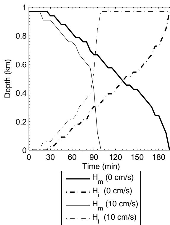
Fig. 5. The variation of the depth of the melting layer (solid lines) and the isothermal layer (dotted lines) in still air (bold) and with the effect of background vertical air velocity of 10 cm/s. H_m refers to the depth of the melting layer and H_i refers to the depth of the isothermal layer at 0°C.
